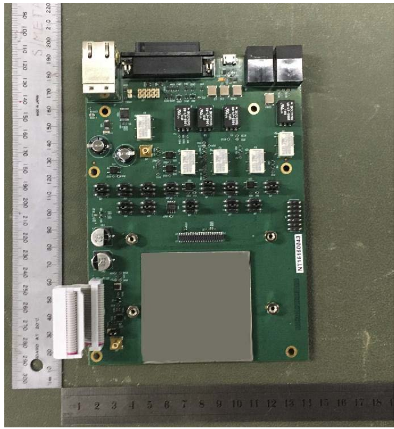
DSP Logic Board Top View
