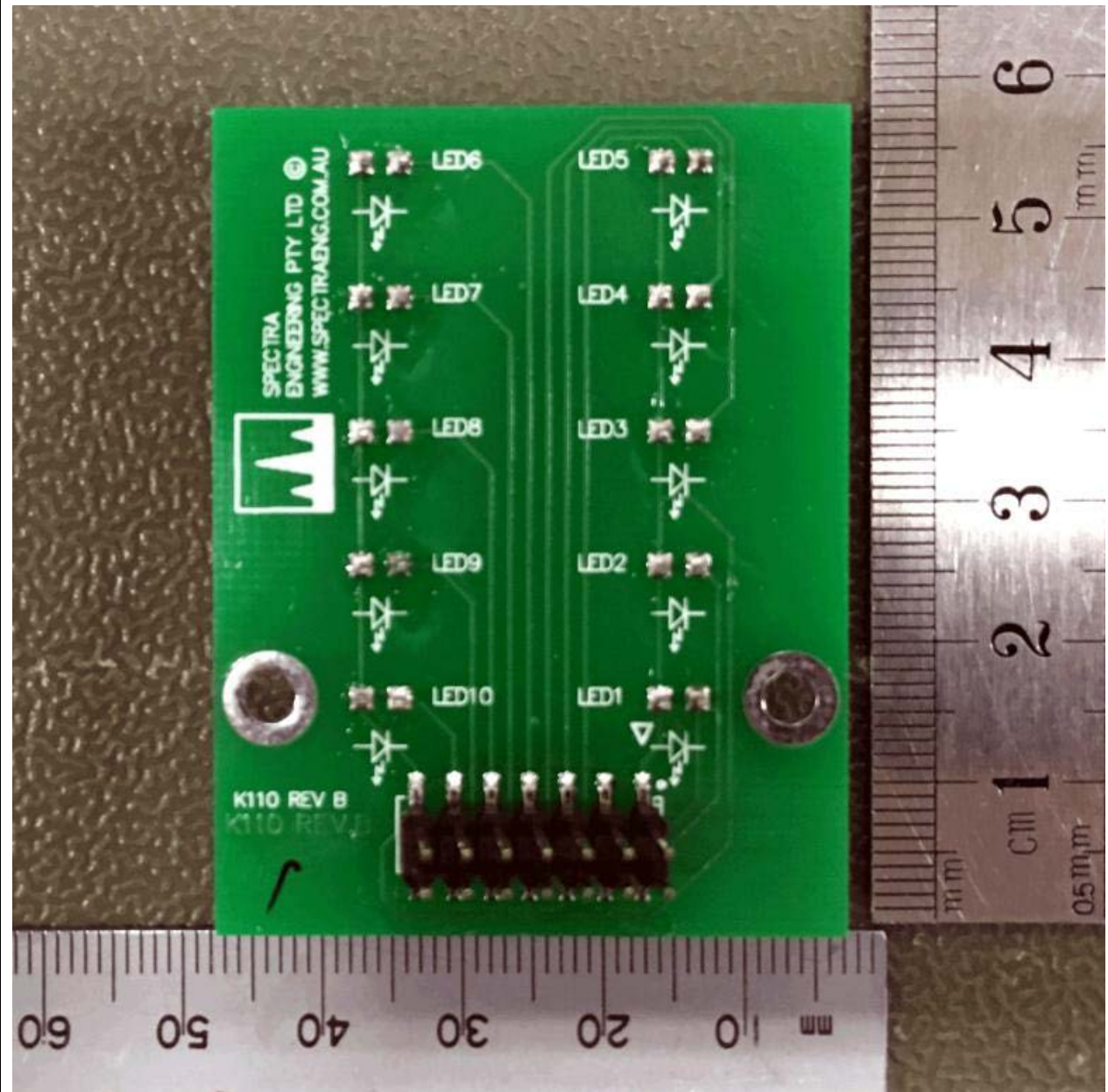
Controller Led PCB Bottom View.
