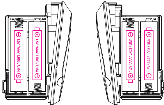
LEFT VIEW
