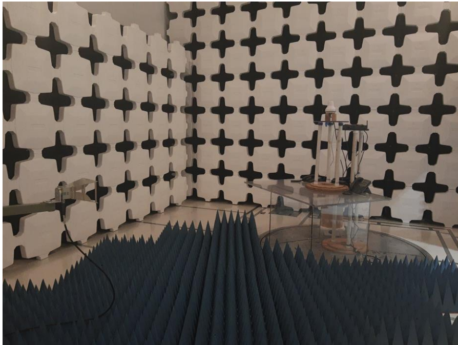
Figure 2: VesseLINK, Radiated Emissions Test Setup, 1-17 GHz
