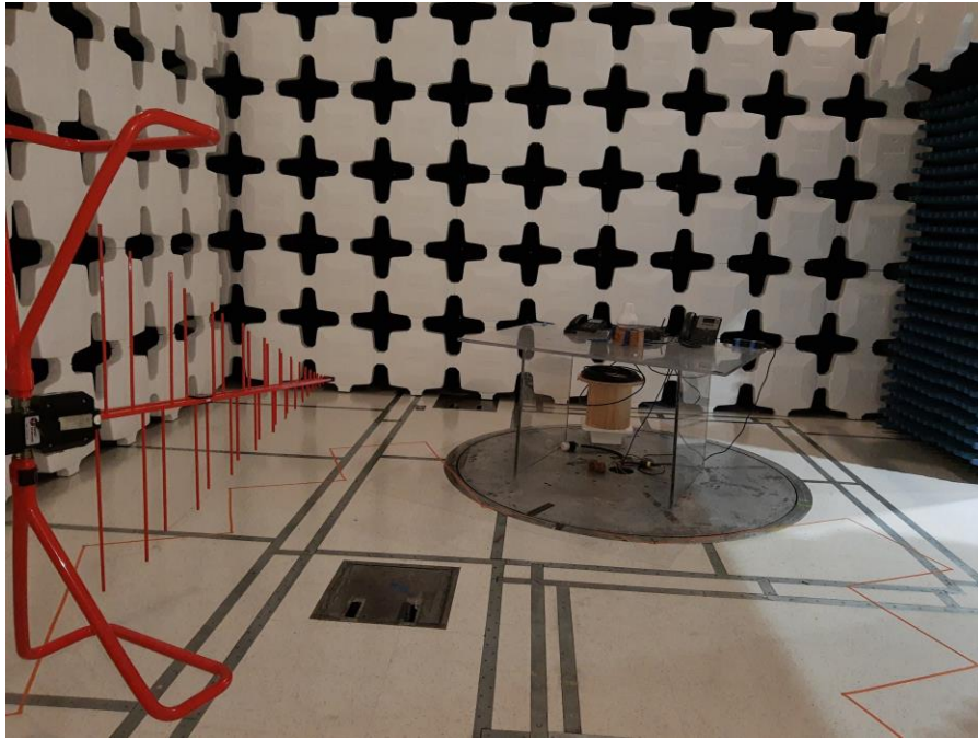
Figure 1: VesseLINK, Radiated Emissions Test Setup, 30-1000 MHz
