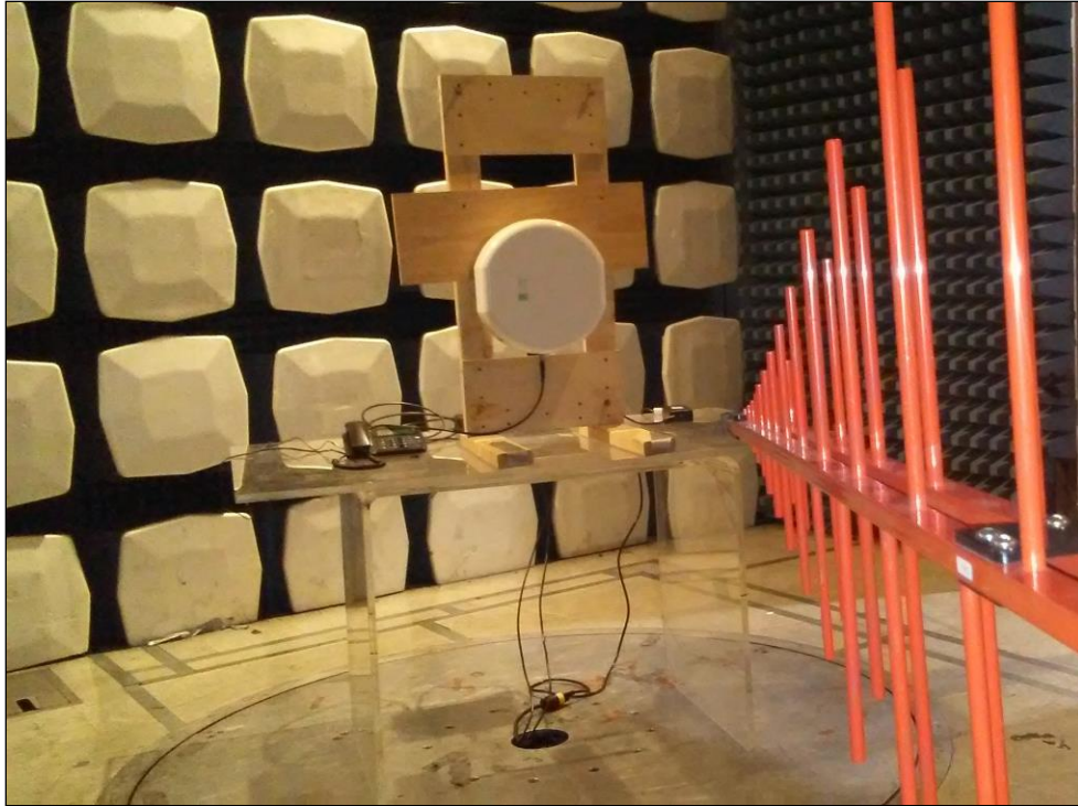
Photograph 1. Radiated Spurious Emissions, Test Setup, Below 1 GHz
