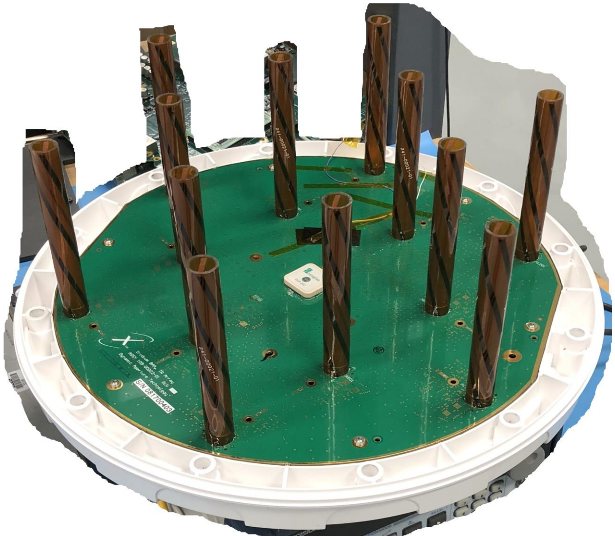
Photograph 2. Antenna Inside
