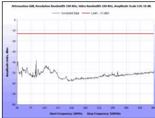
Plot 23. Radiated Spurious Emissions, M424, Channel 1, 1616.333 MHz, 30 MHz – 500 MHz
