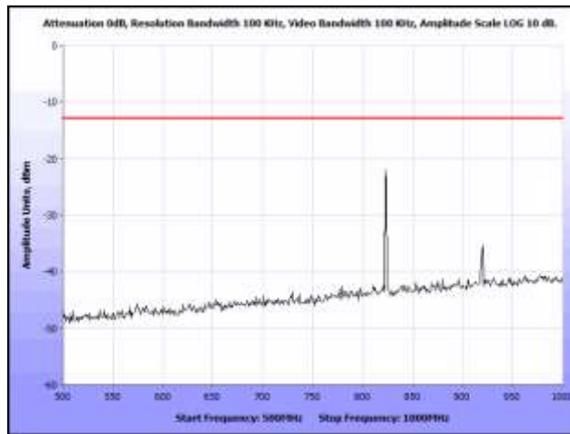
Plot 36. Radiated Spurious Emissions, M424, Channel 232, 1625.666 MHz, 500 MHz – 1 GHz
