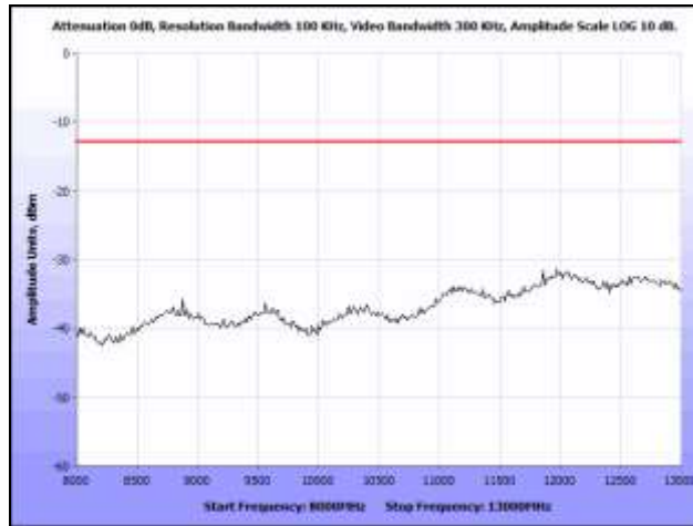
Plot 39. Radiated Spurious Emissions, M424, Channel 232, 1625.666 MHz, 8 GHz – 13 GHz
