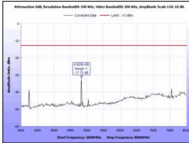
Plot 32. Radiated Spurious Emissions, M424, Channel 121, 1621.333 MHz, 3 GHz – 8 GHz
