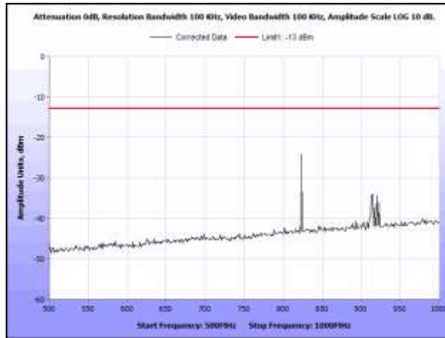
Plot 30. Radiated Spurious Emissions, M424, Channel 121, 1621.333 MHz, 500 MHz – 1 GHz
