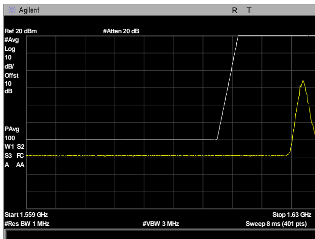
Plot 3. Aeronautical Radio Protection, EIRP, M424, Channel 232, 1625.666 MHz
