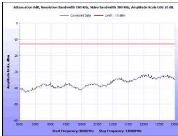
Plot 27. Radiated Spurious Emissions, M424, Channel 1, 1616.333 MHz, 8 GHz – 13 GHz
