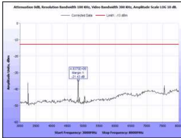
Plot 38. Radiated Spurious Emissions, M424, Channel 232, 1625.666 MHz, 3 GHz – 8 GHz
