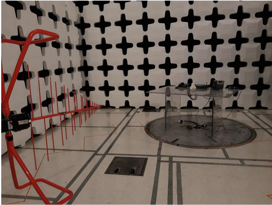
Figure 1: MissionLINK, Radiated Emissions Test Setup, 30-1000 MHz
