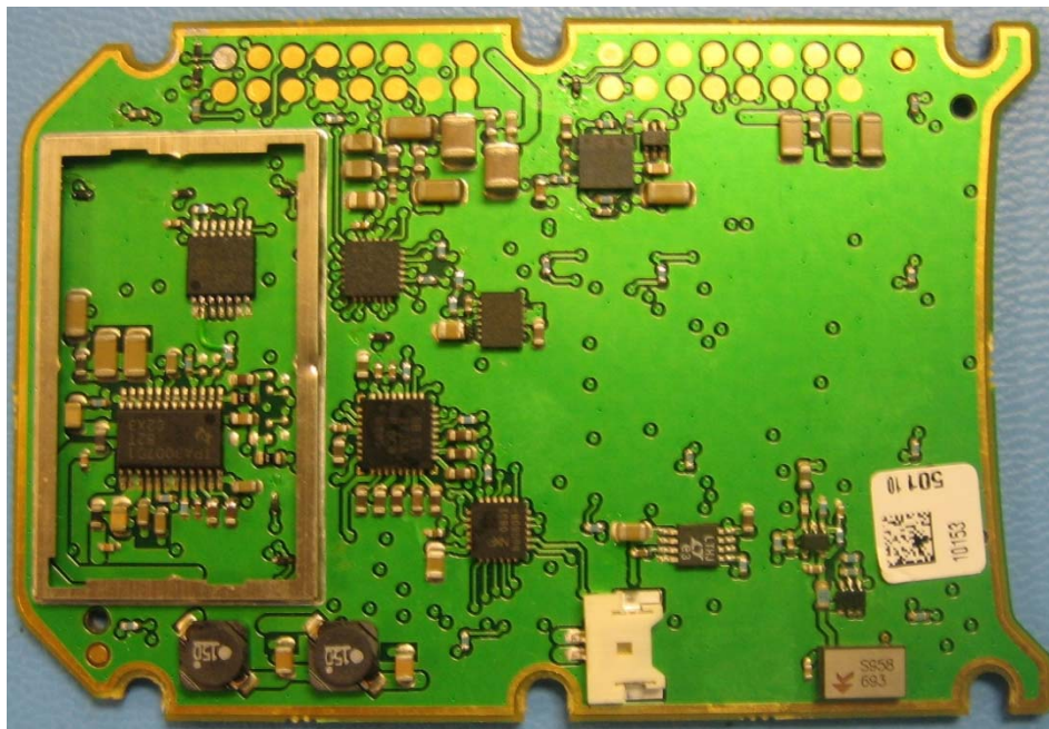
Figure 9 – 4102010-501, Keypad PWB Bottom (Without Shield Lids)
