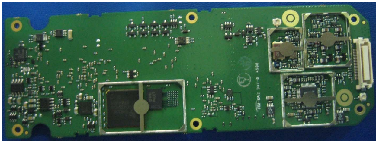
Figure 6 – 4102013-501, Control PWB Bottom (Without Shield Lids)
