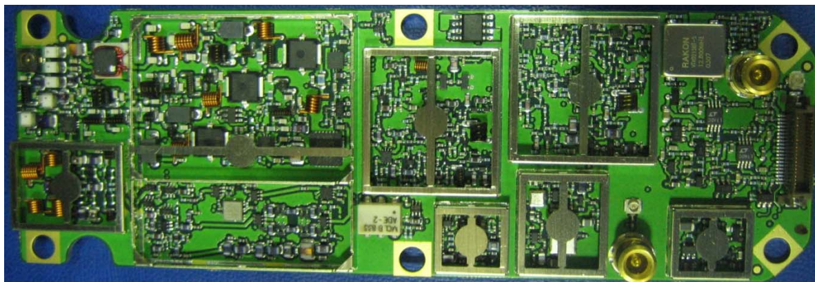
Figure 1 – 4102056-501, XCVR PWB Top (Without Shield Lids)
