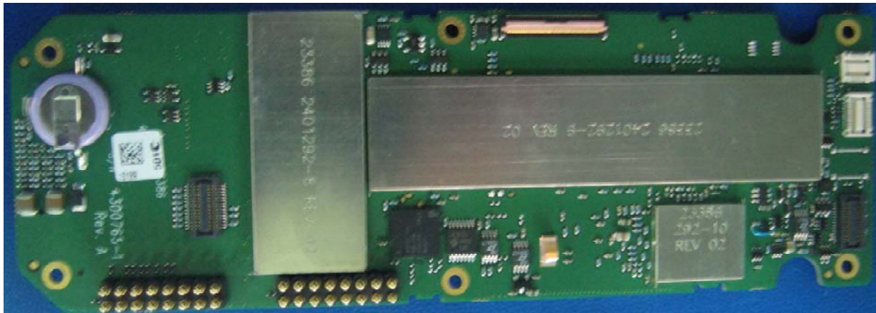
Figure 5 – 4102013-501, Control PWB Top (With Shield Lids)
