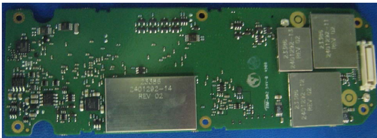
Figure 7 – 4102013-501, Control PWB Bottom (With Shield Lids)
