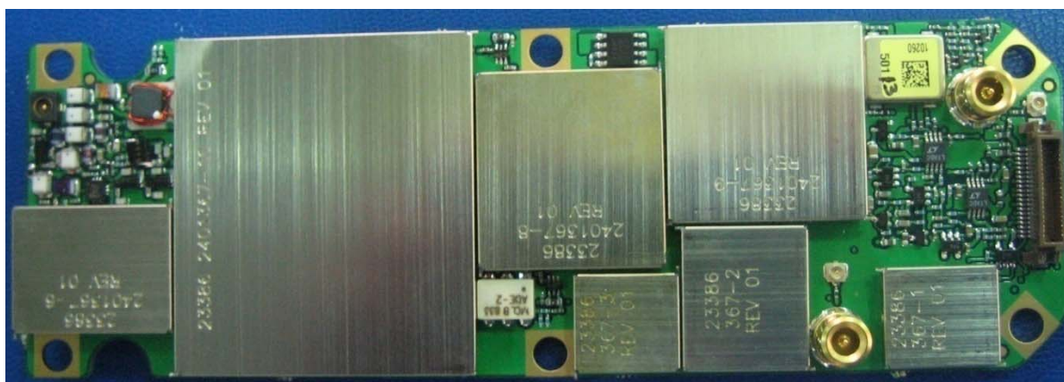
Figure 2 – 4102056-501, XCVR PWB Top (With Shield Lids)
