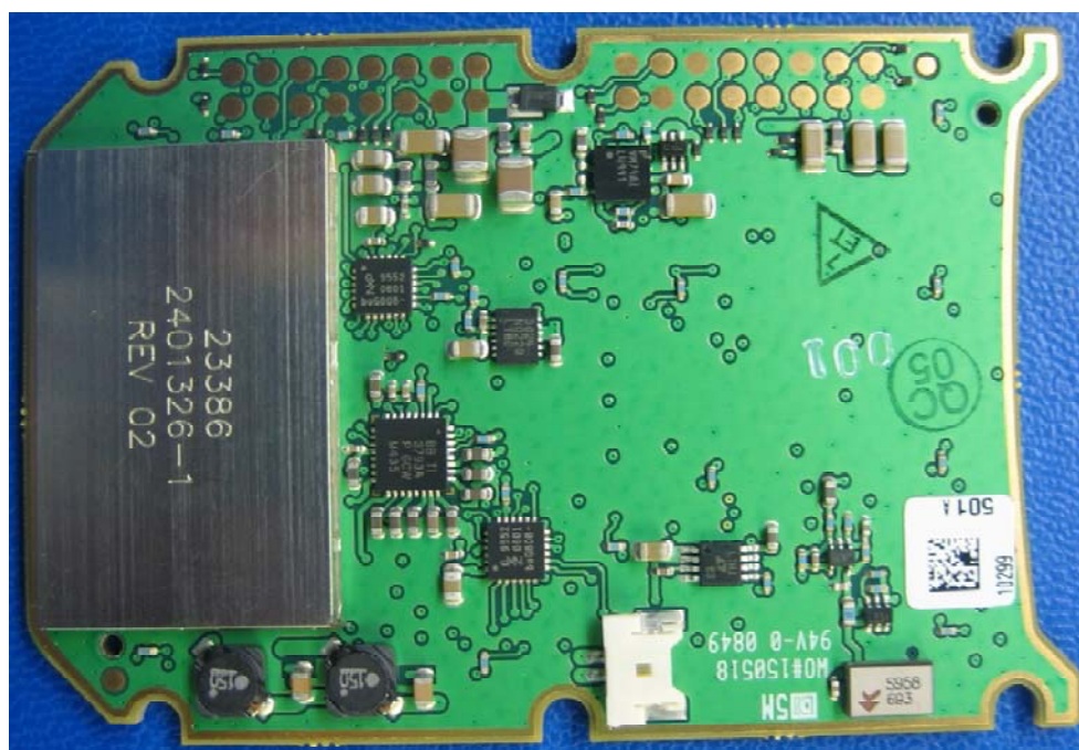
Figure 10 – 4102010-501, Keypad PWB Bottom (With Shield Lids)
