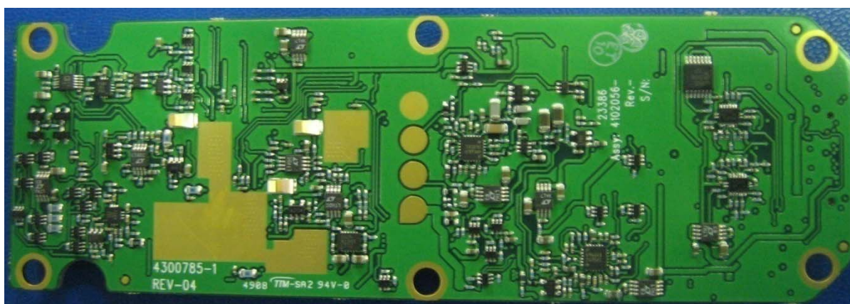
Figure 3 – 4102056-501, XCVR PWB Bottom
