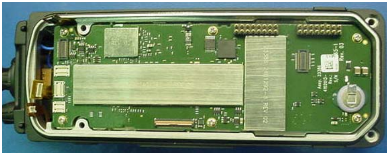
Figure 16 – View of Control PWB (4102013-501) installed over the XCVR PWB (4102056-501) and inner shield assemblies.
