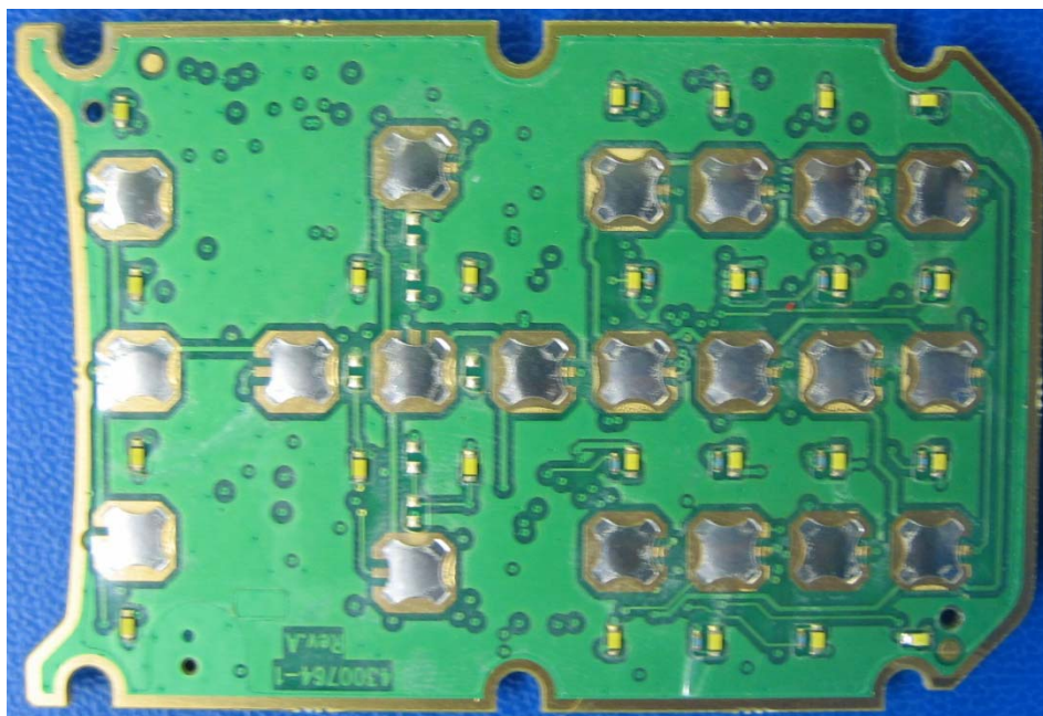
Figure 8 – 4102010-501, Keypad PWB Top
