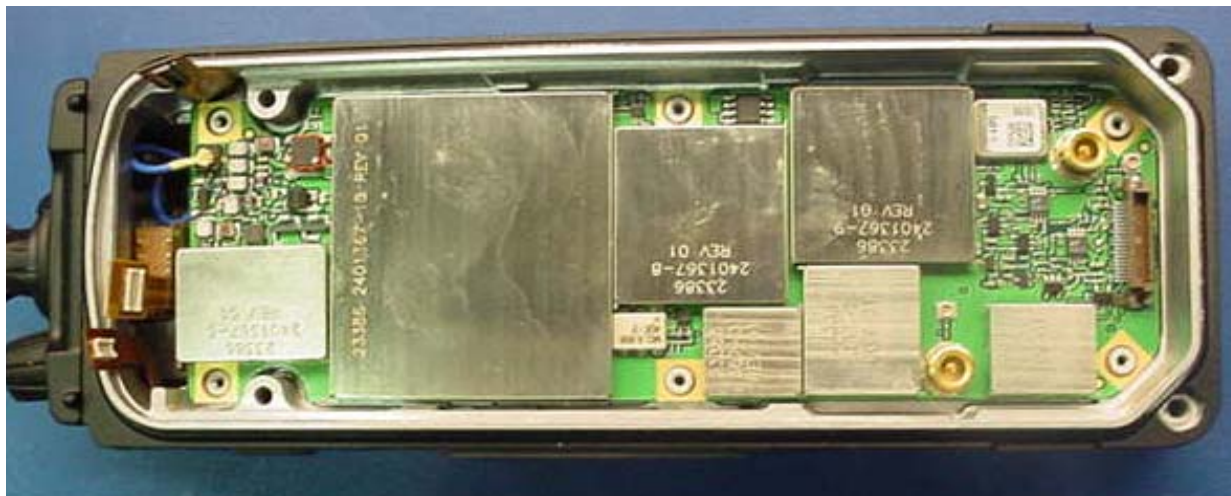
Figure 14 – View of XCVR PWB (4102056-501) installation into radio chassis.
