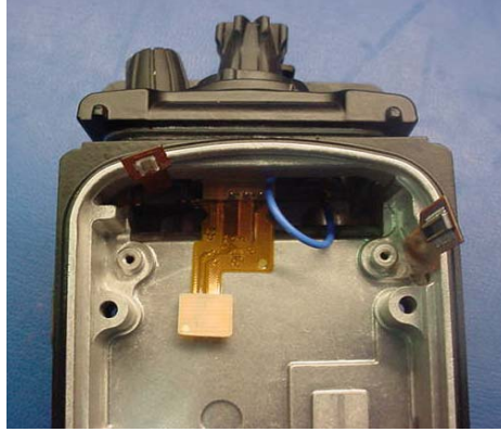
Figure 11 – View of Chassis Top Plate assembly with the radio chassis.
