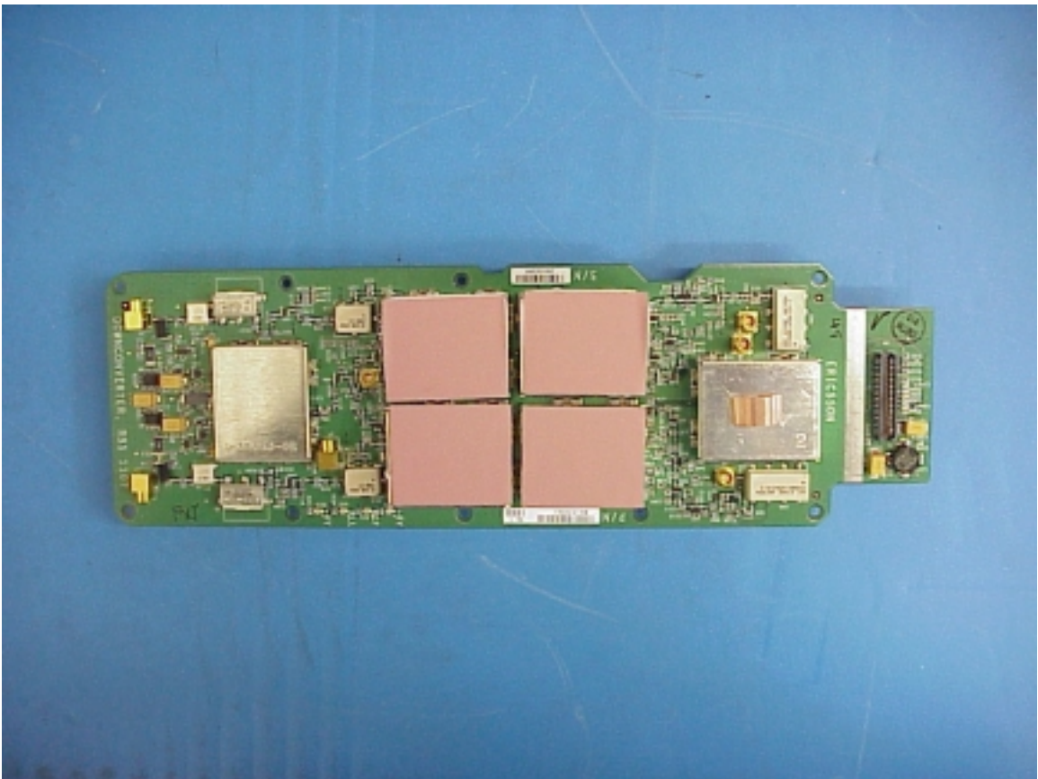
Downconverter Board
