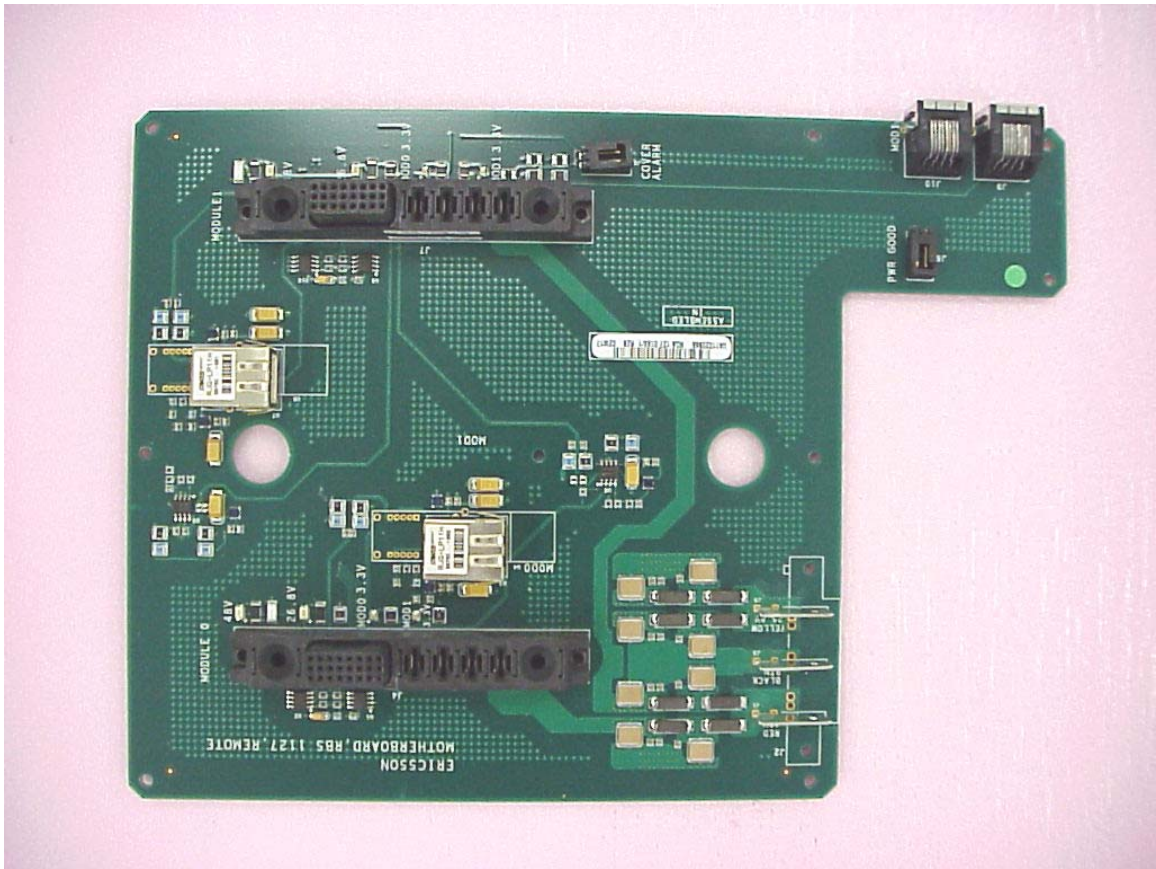
RBS1127 PLR Mother Board Top-Side
