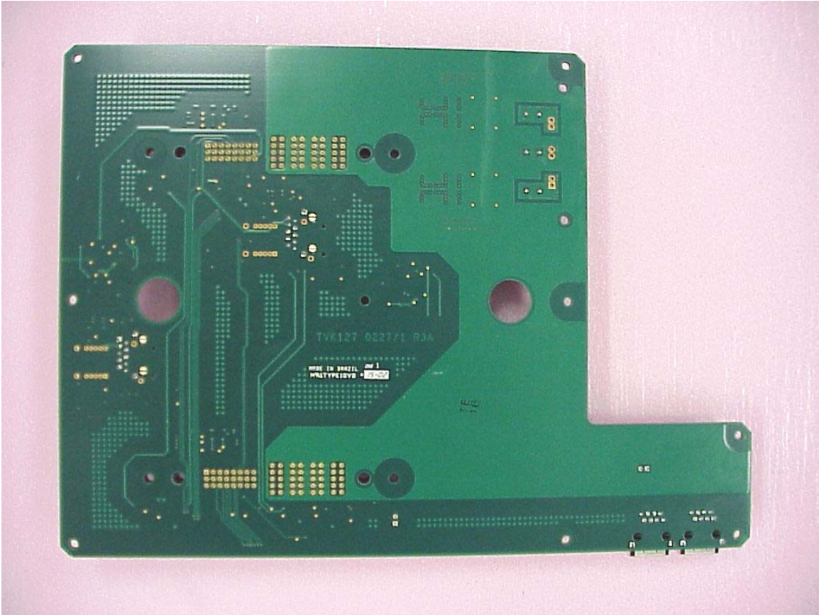
RBS1127 PLR Mother Board Bottom-Side
