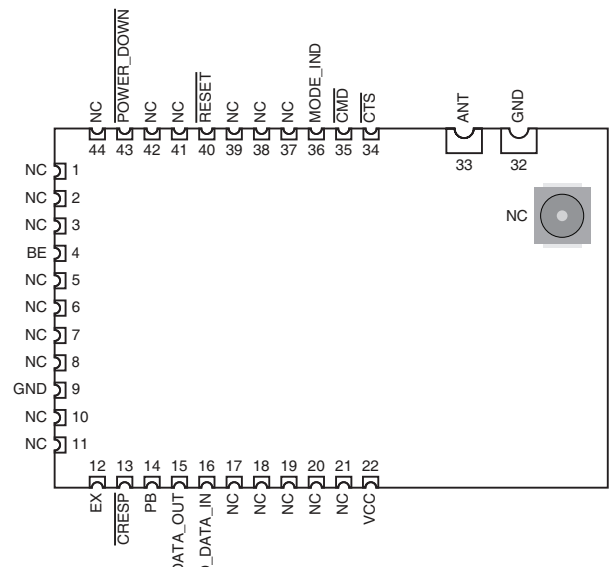
Figure 16: HumPRO-A™ Series Transceiver Pre-certified Version Pin Assignments - Castellated Connection (Top View)
