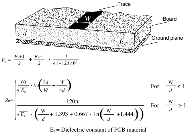
Figure 110: Microstrip Formulas
