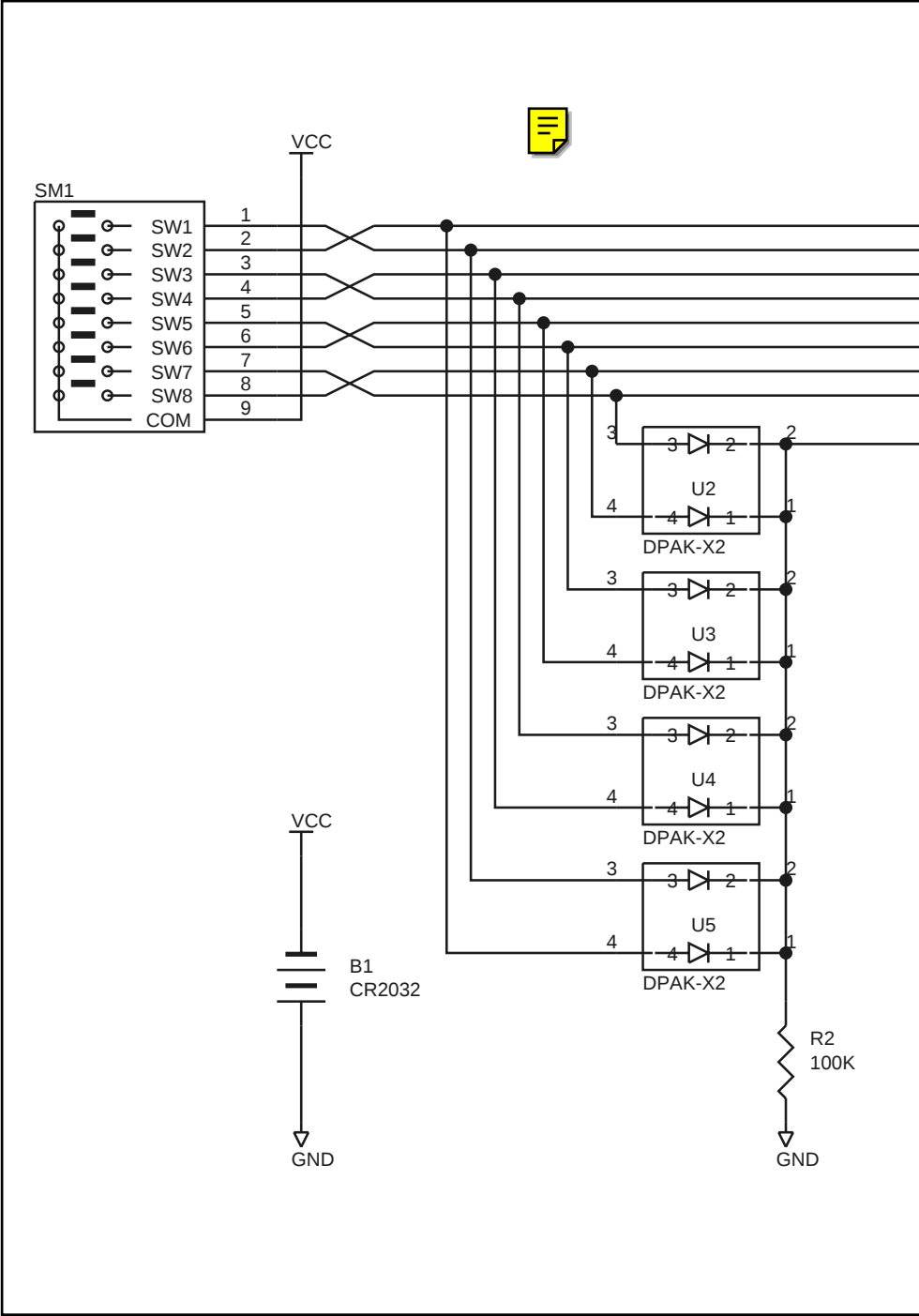
HHLR Schematic
