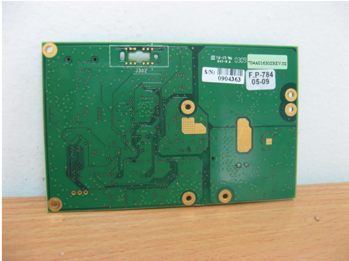
POD Board Print side
