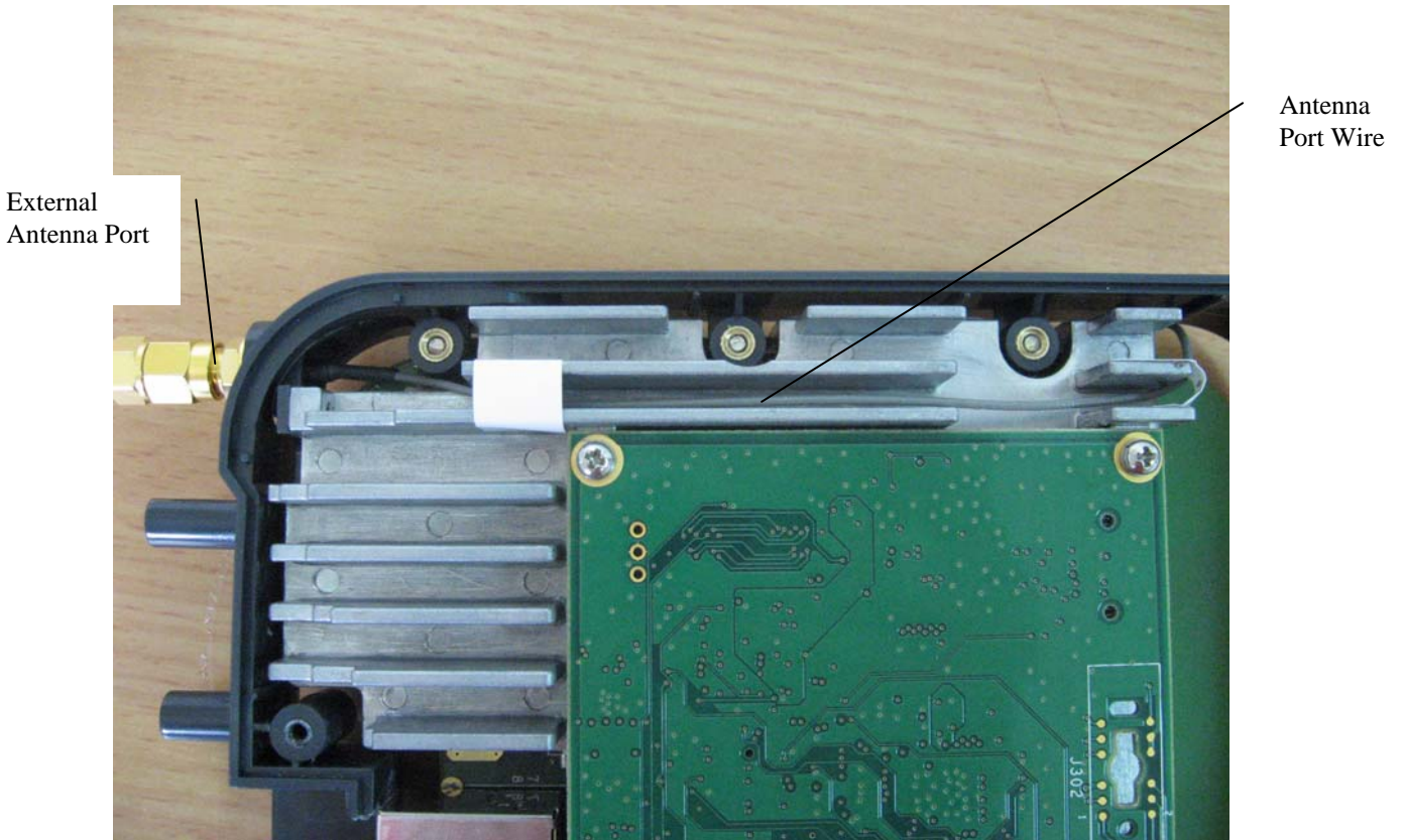
RF Board Side 2
