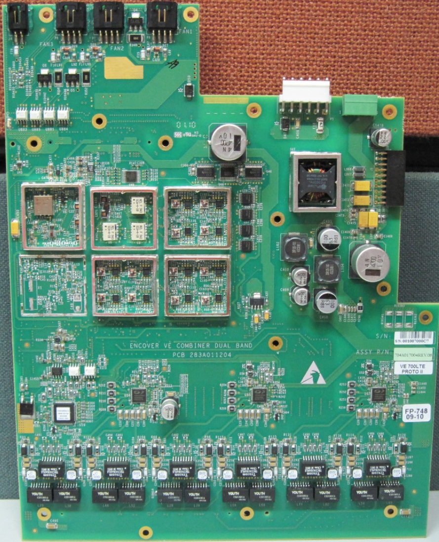
Combiner Side 1
