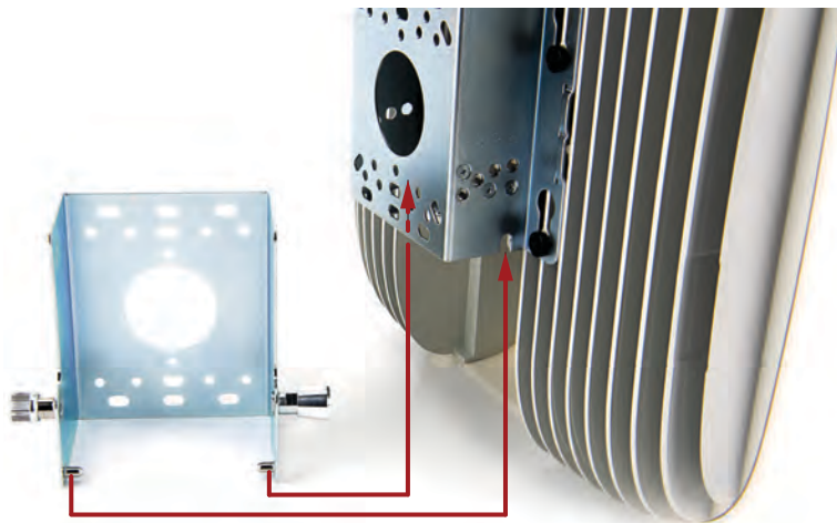
Figure 10 Attaching the SCR N-520 with Ceiling-Mount Bracket to the Wall-Mount Bracket
