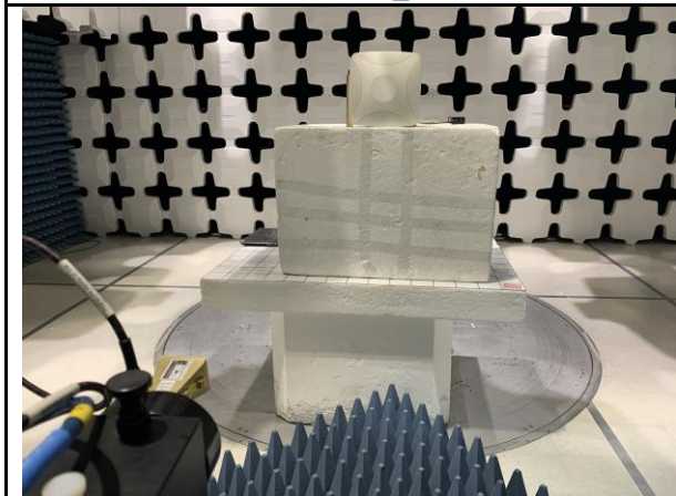
Radiated Emission Test Above 18GHz-50GHz Front View_2m
