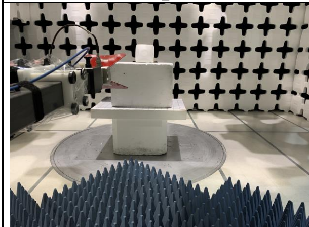
Radiated Emission Test Above 1GHz-18GHz Front View_3m
