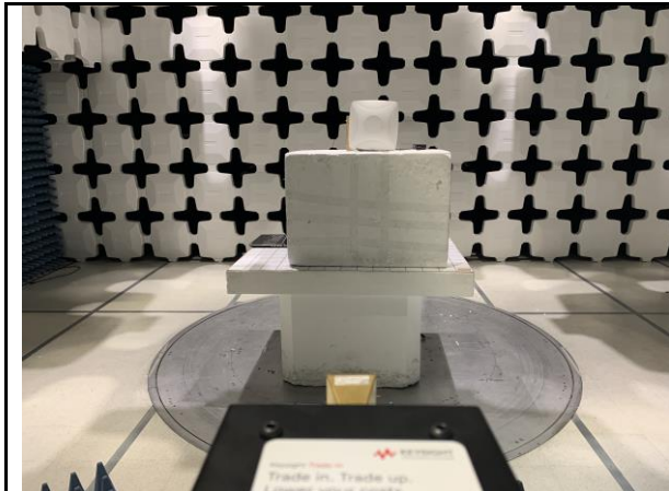
Radiated Emission Test Above 50GHz-75GHz Front View_3m
