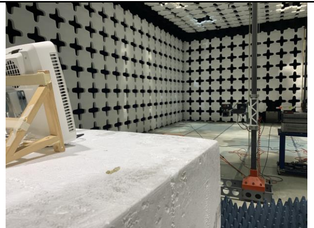
Radiated Emission Test Above 50GHz-75GHz Rear View_3m
