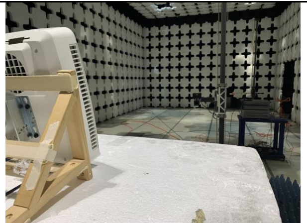
Radiated Emission Test Above 75GHz-100GHz Rear View_3m
