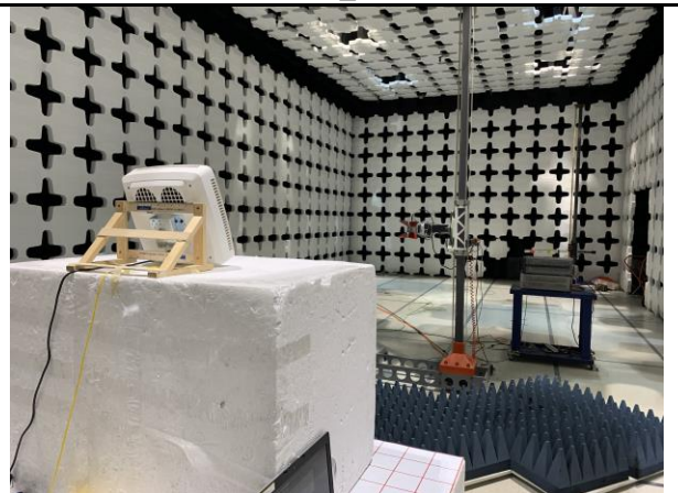
Radiated Emission Test Above 1GHz-18GHz Rear View_3m
