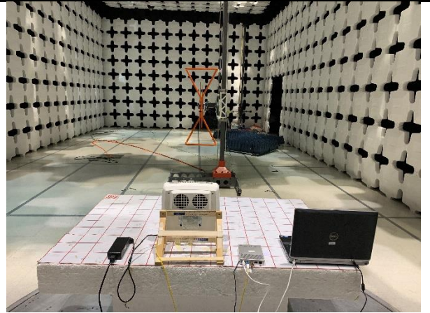
Radiated Emission Test below 1GHz Rear View_3m
