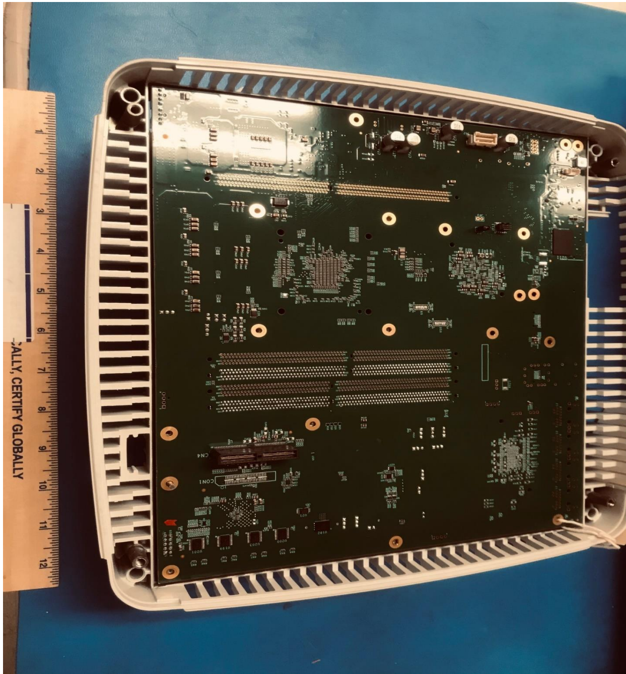
NXP Board
