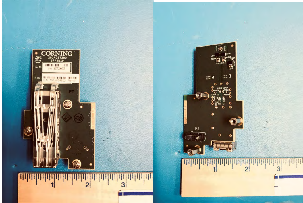
SFP2NXP board
