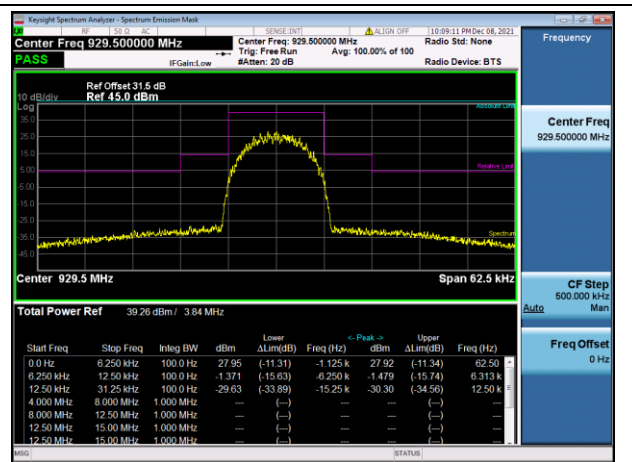
25kHz TETRA
