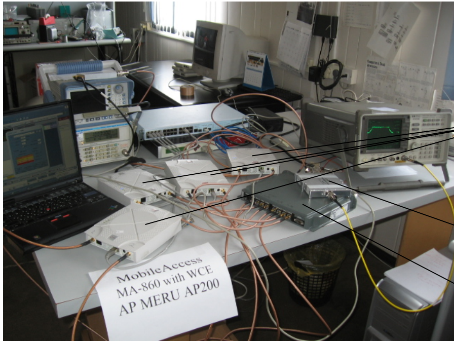
Conducted Emission on Antenna Port
