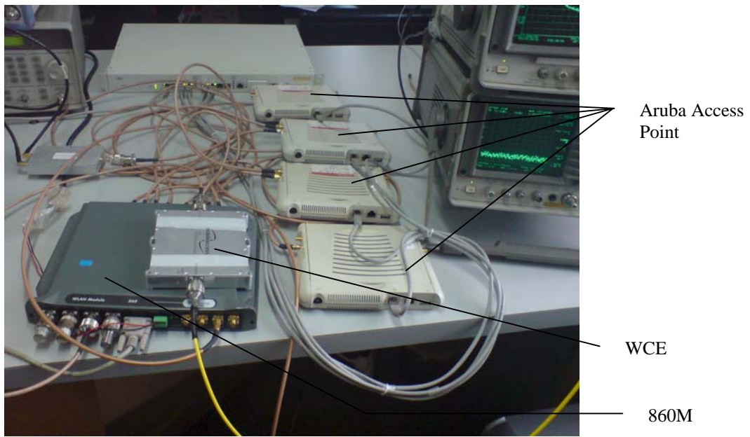
Conducted Emission From antenna Ports Close-up
