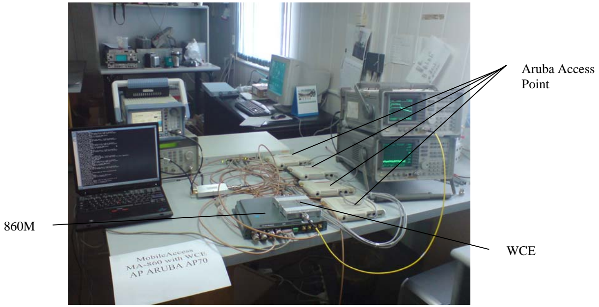
Conducted Emissions From Antenna Ports
