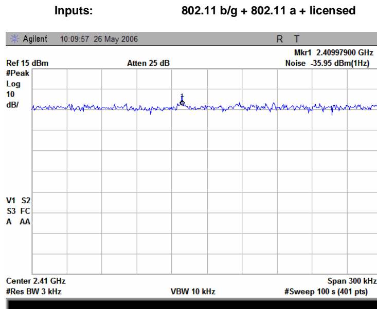
Plot 7.7.50 Peak spectral power density at low frequency zoomed at the peak at 1 Mbps DSSS
