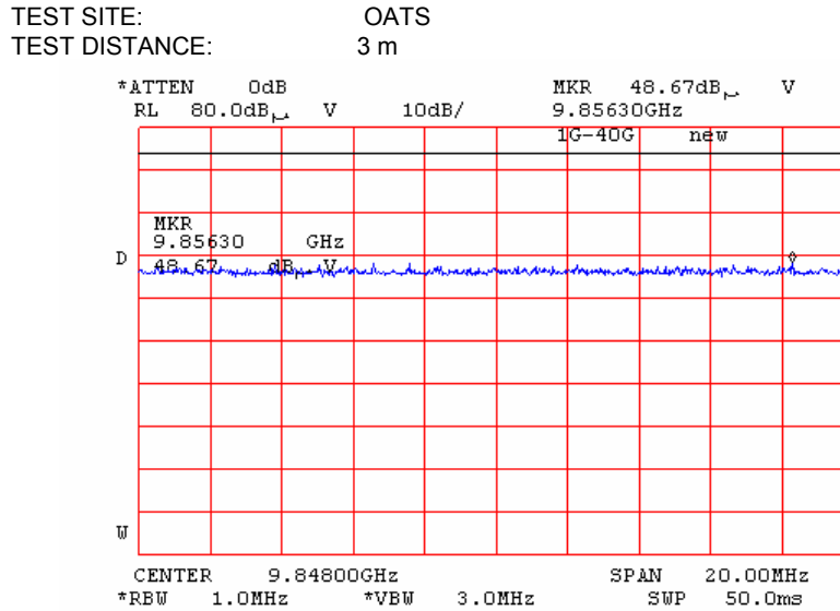
Plot 7.5.70 Radiated emission measurements at the fourth harmonic of high carrier frequency
