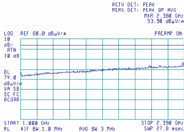
Plot 7.5.17 Radiated emission measurements from 1000 to 2390 MHz at the high carrier frequency
