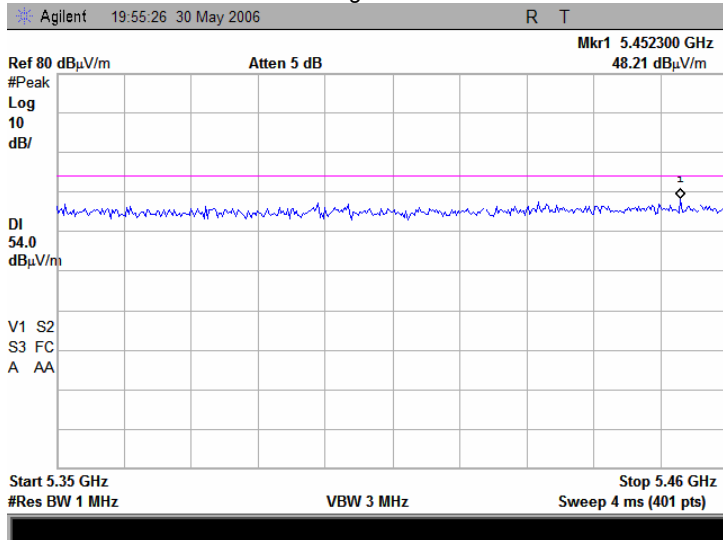
Plot 7.5.37 Radiated emission measurements from 5350 to 5460 MHz at the mid carrier frequency
