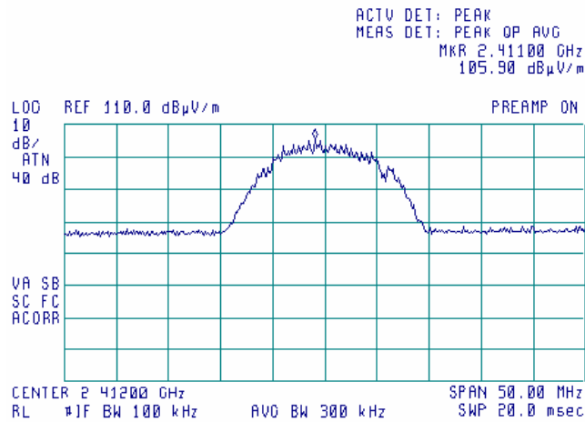
Plot 7.6.2 Radiated emission measurements at the low carrier frequency
