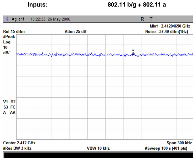
Plot 7.7.32 Peak spectral power density at low frequency zoomed at the peak at 11 Mbps DSSS
