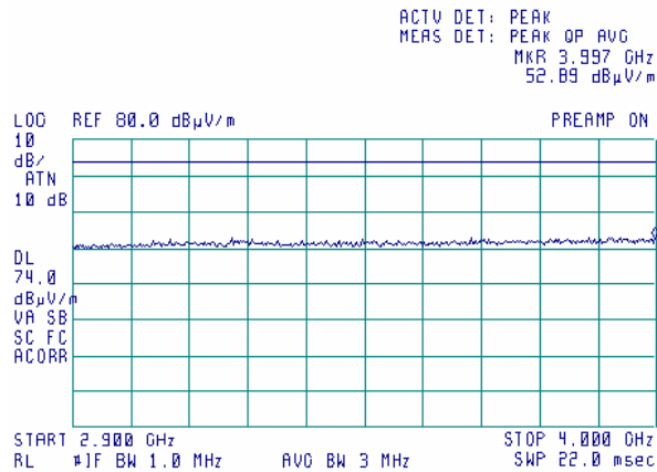
Plot 7.6.43 Radiated emission measurements from 2900 to 4000 MHz at the high carrier frequency
