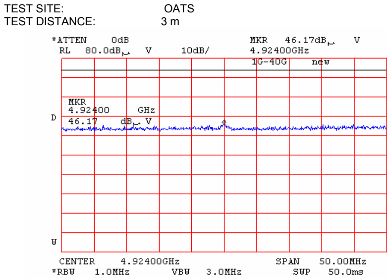
Plot 7.5.133 Radiated emission measurements at the second harmonic of high carrier frequency
