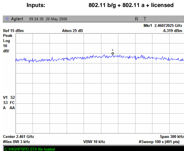
Plot 7.7.72 Peak spectral power density at high frequency zoomed at the peak at 54 Mbps OFDM
