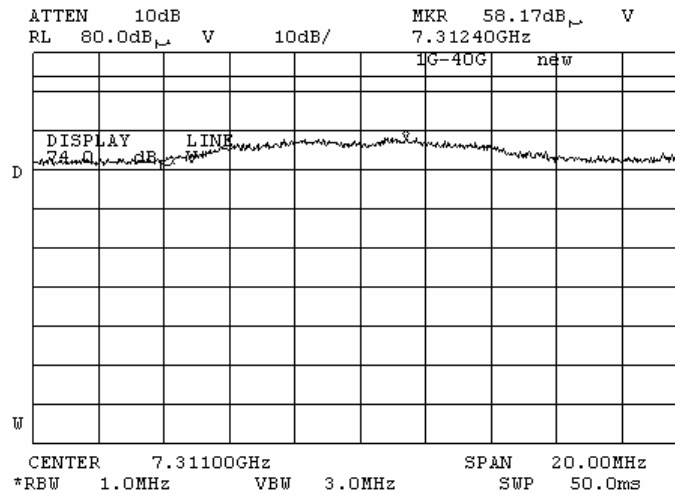
Plot 7.6.76 Radiated emission measurements at the third harmonic of mid carrier frequency
