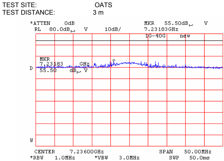
Plot 7.5.134 Radiated emission measurements at the third harmonic of low carrier frequency
