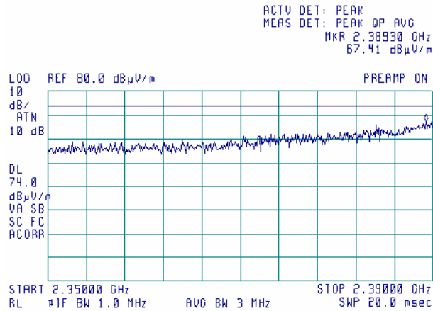
Plot 7.6.19 Radiated emission measurements from 2350 to 2390 MHz at the low carrier frequency
