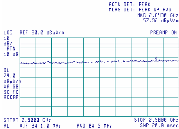
Plot 7.6.31 Radiated emission measurements from 2500 to 2900 MHz at the low carrier frequency
