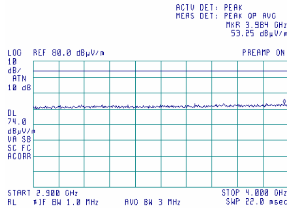
Plot 7.6.39 Radiated emission measurements from 2900 to 4000 MHz at the low carrier frequency
