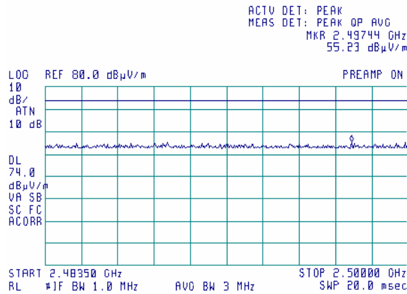
Plot 7.5.90 Radiated emission measurements from 2483.5 to 2500 MHz at the low carrier frequency
