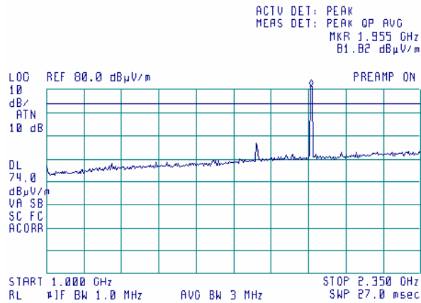
Plot 7.5.82 Radiated emission measurements from 1000 to 2350 MHz at the low carrier frequency
