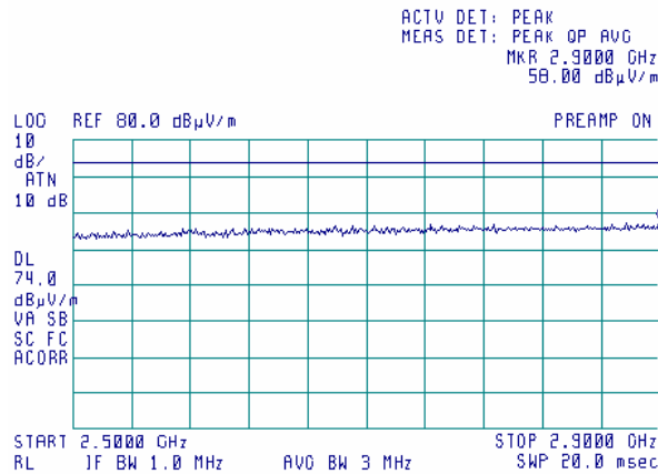
Plot 7.5.98 Radiated emission measurements from 2500 to 2900 MHz at the mid carrier frequency
