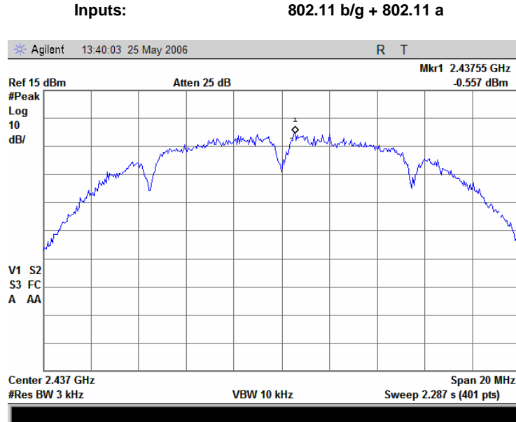
Plot 7.7.28 Peak spectral power density at mid frequency zoomed at the peak at 1 Mbps DSSS
