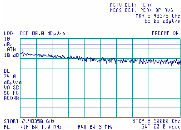
Plot 7.6.29 Radiated emission measurements from 2483.5 to 2500 MHz at the high carrier frequency
