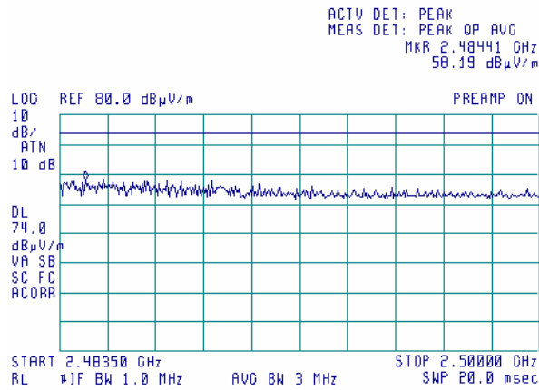
Plot 7.6.27 Radiated emission measurements from 2483.5 to 2500 MHz at the mid carrier frequency
