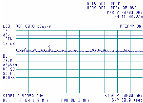
Plot 7.5.92 Radiated emission measurements from 2483.5 to 2500 MHz at the mid carrier frequency
