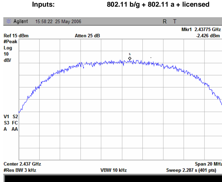
Plot 7.7.58 Peak spectral power density at mid frequency zoomed at the peak at 11 Mbps DSSS
