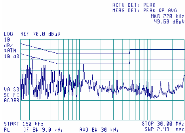
Plot 7.8.2 Conducted emission measurements A.C mains to MA850
