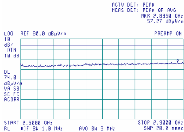
Plot 7.6.33 Radiated emission measurements from 2500 to 2900 MHz at the mid carrier frequency
