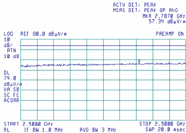
Plot 7.5.100 Radiated emission measurements from 2500 to 2900 MHz at the high carrier frequency
