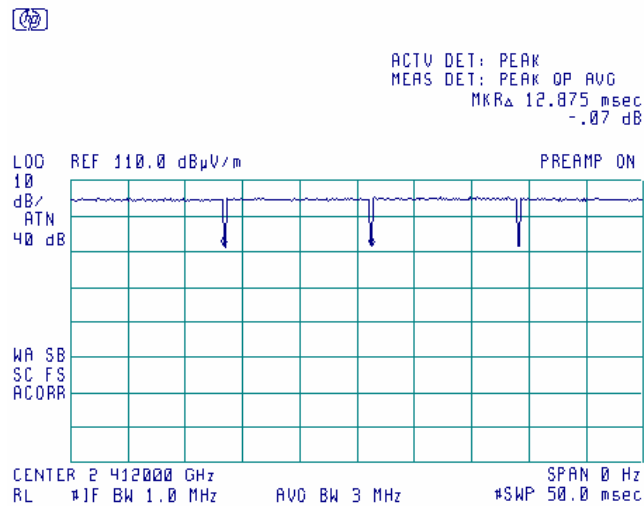
Plot 7.5.71 Transmission pulse duration
