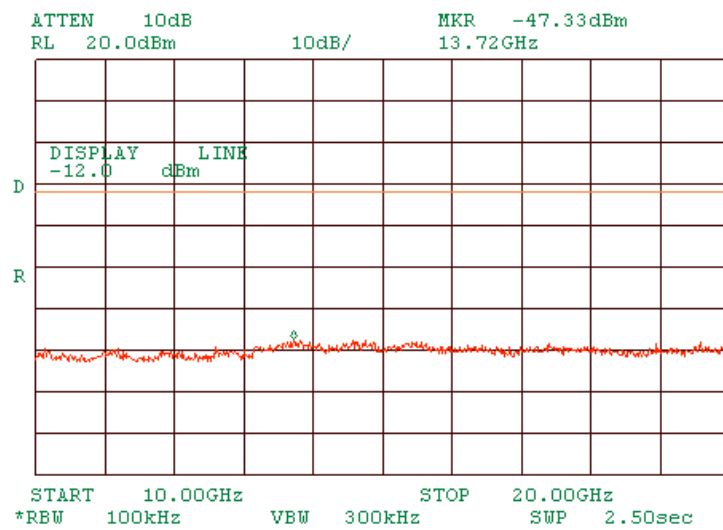
Plot 1.7.25 Spurious emission measurements in 10000 - 20000 MHz range at low carrier frequency DSSS
