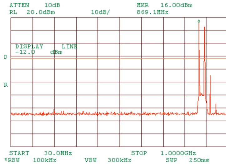
Plot 1.7.12 Spurious emission measurements in 30 - 1000 MHz range at mid carrier frequency DSSS
