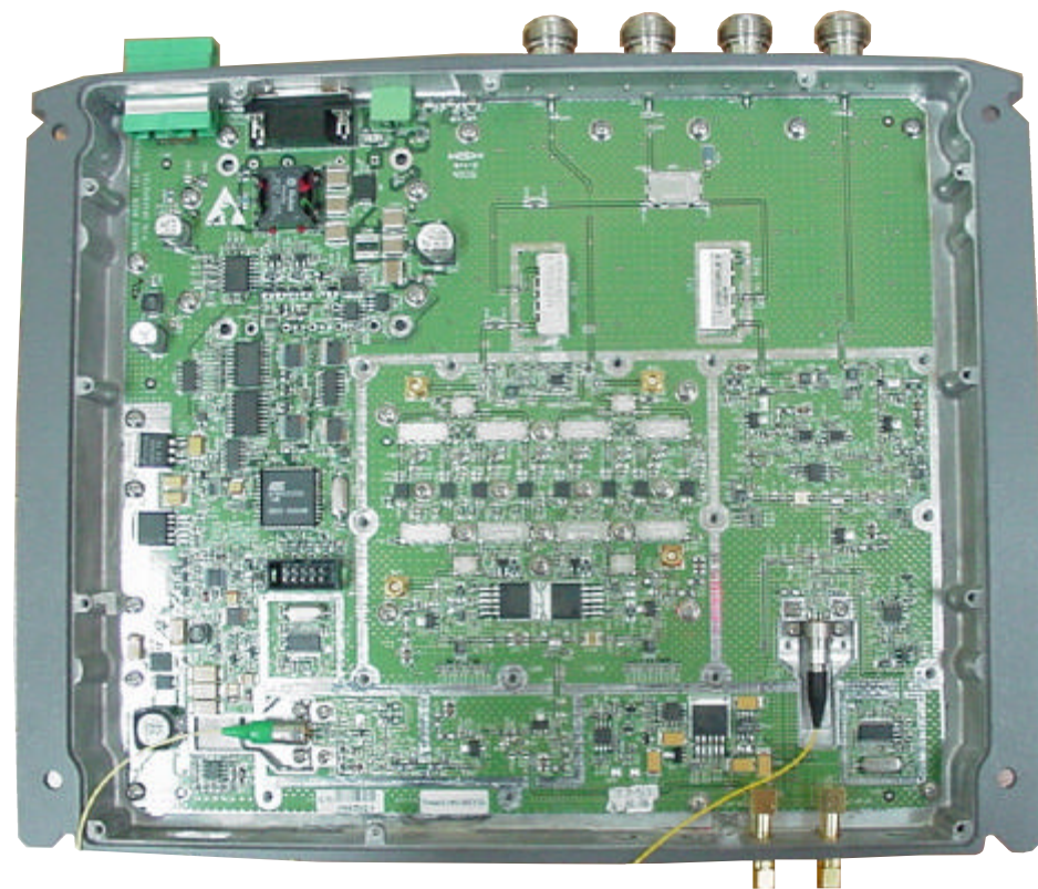
2000-IDEN-SMRE - Unit after change, with an without shield
