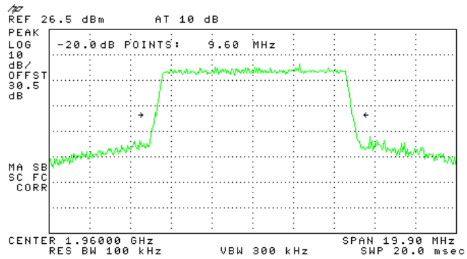
Figure 74.— 1960 MHz
