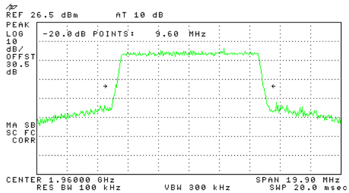
Figure 77.— 1960 MHz
