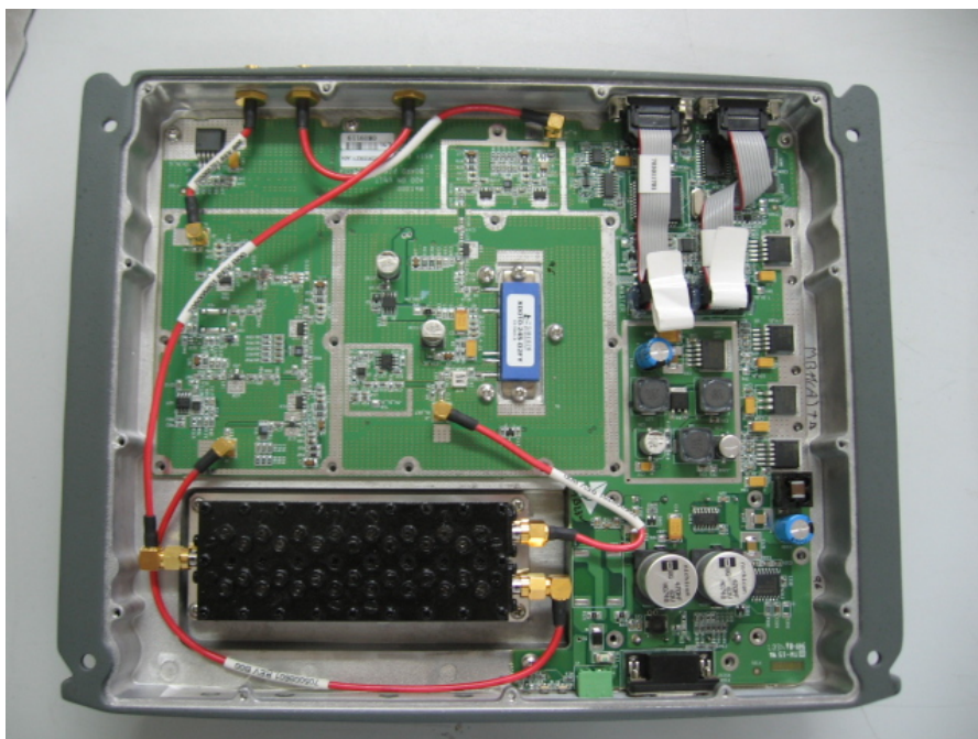
PCB Without Shield In Cover
