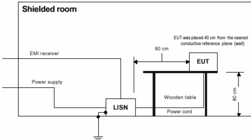
Setup for mains terminal radio interference voltage test, table-top equipment
