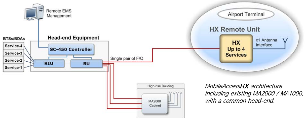
Figure 1-2. System Architecture
