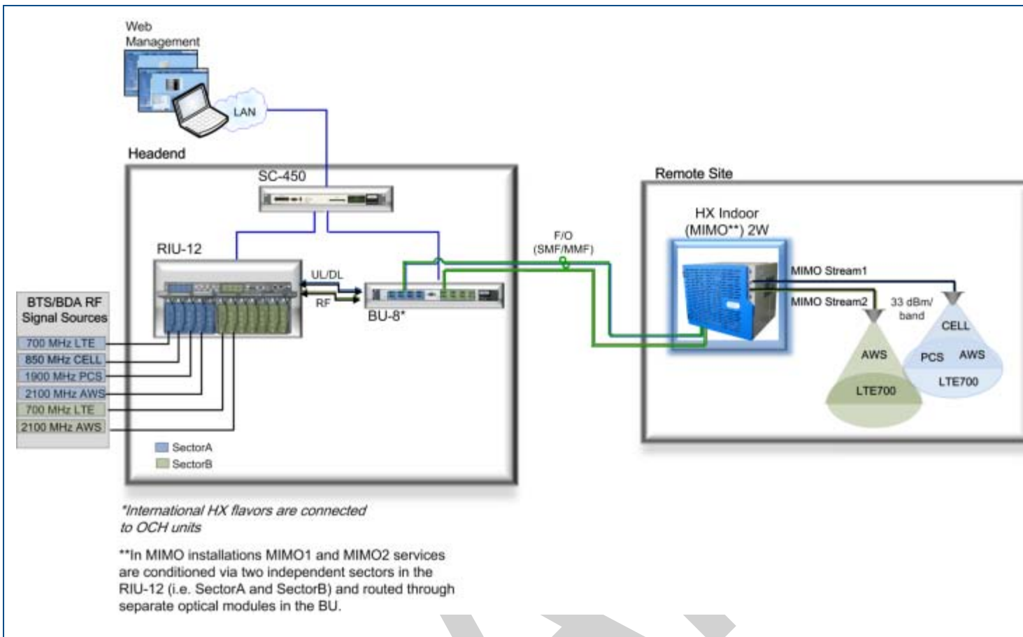
Example of Indoor MIMO Architecture with HX Quad-Band
