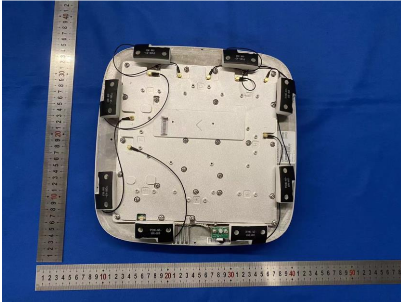
Internal Antenna
