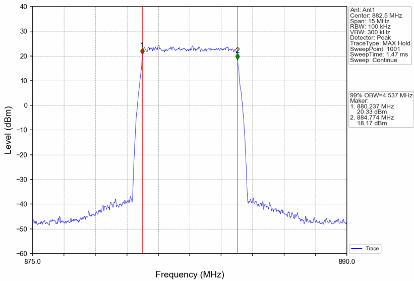
Band26b_882.5MHz_AWGN_SISO_Ant1_NTNV_AGC
