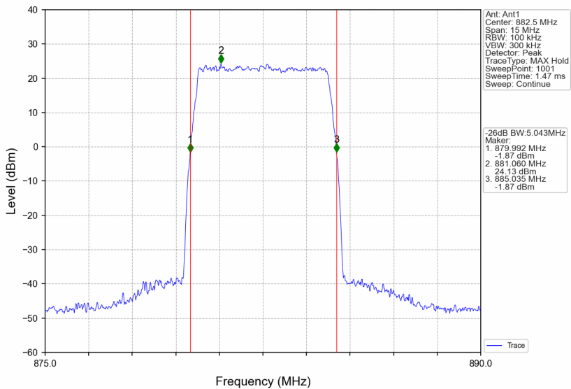
Band26b_882.5MHz_AWGN_SISO_Ant1_NTNV_AGC
