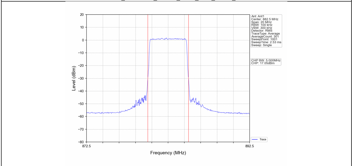
Band26b_882.5MHz_AWGN_SISO_Ant1_NTNV_AGC+3
