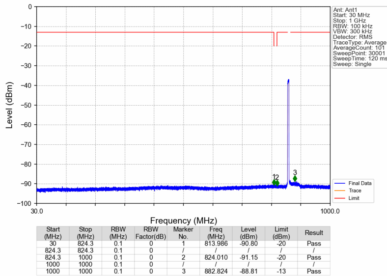
Band26a_861.5MHz_AWGN_SISO_Ant1_NTNV
