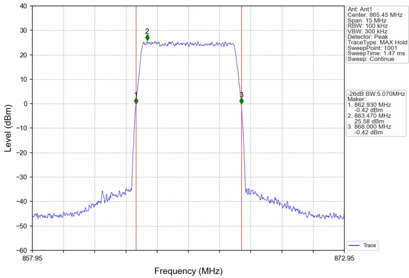
Band26a_865.45MHz_AWGN_SISO_Ant1_NTNV_AGC
