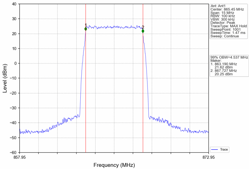
Band26a_865.45MHz_AWGN_SISO_Ant1_NTNV_AGC
