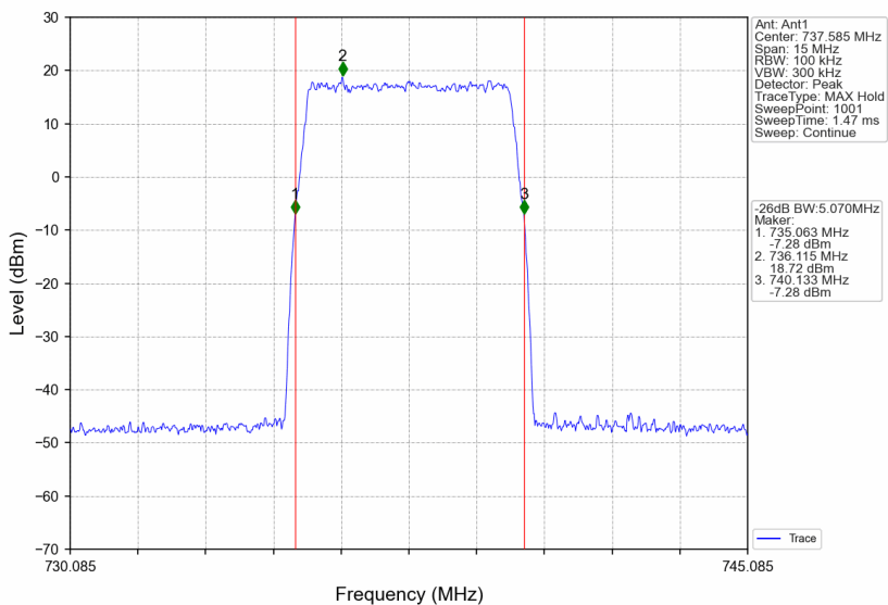
Band12_737.585MHz_AWGN_SISO_Ant1_NTNV_AGC
