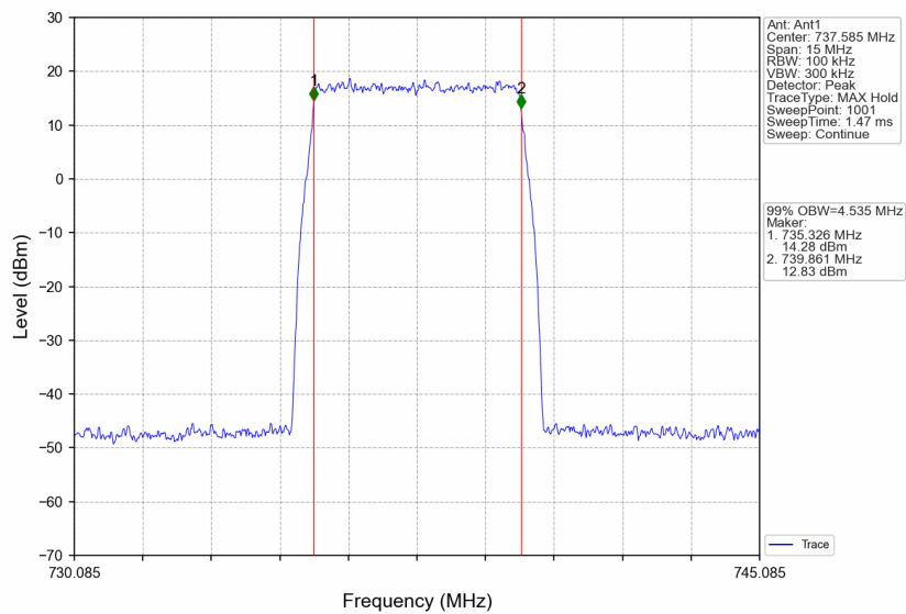
Band12_737.585MHz_AWGN_SISO_Ant1_NTNV_AGC
