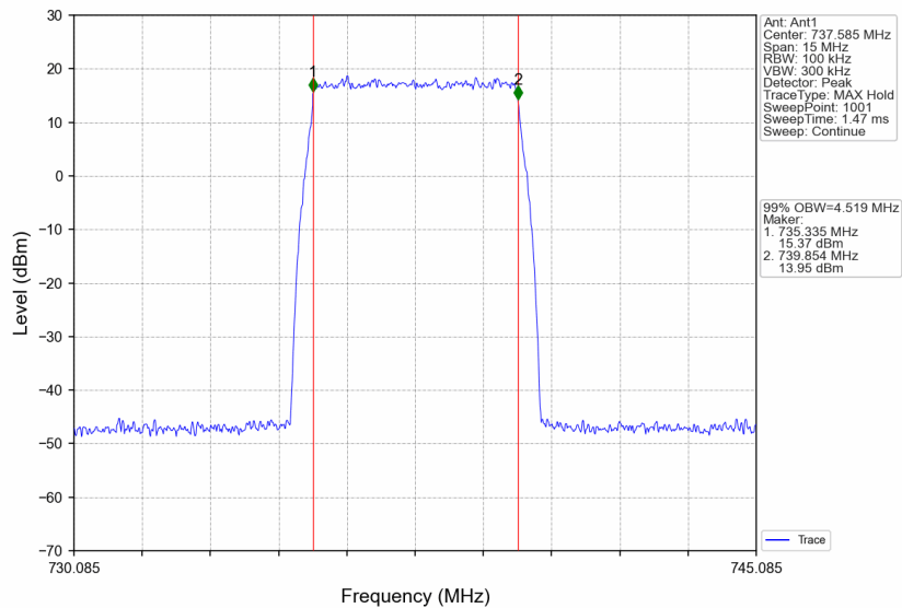
Band12_737.585MHz_AWGN_SISO_Ant1_NTNV_AGC
