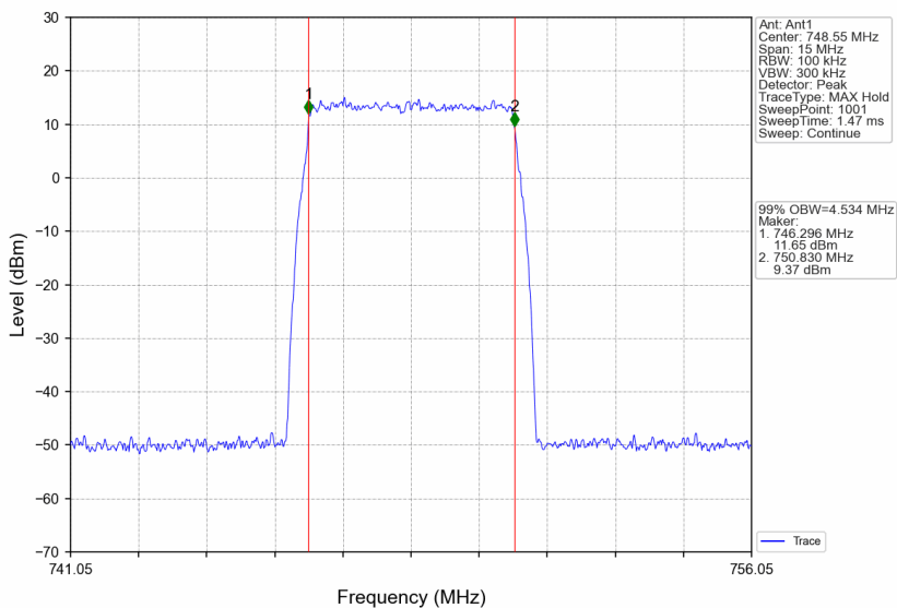
Band13_748.55MHz_AWGN_SISO_Ant1_NTNV_AGC
