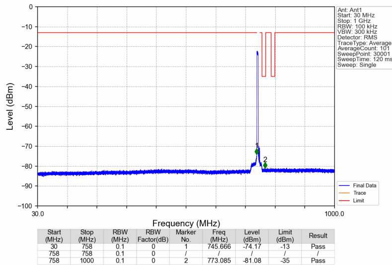
Band13_748.5MHz_AWGN_SISO_Ant1_NTNV
