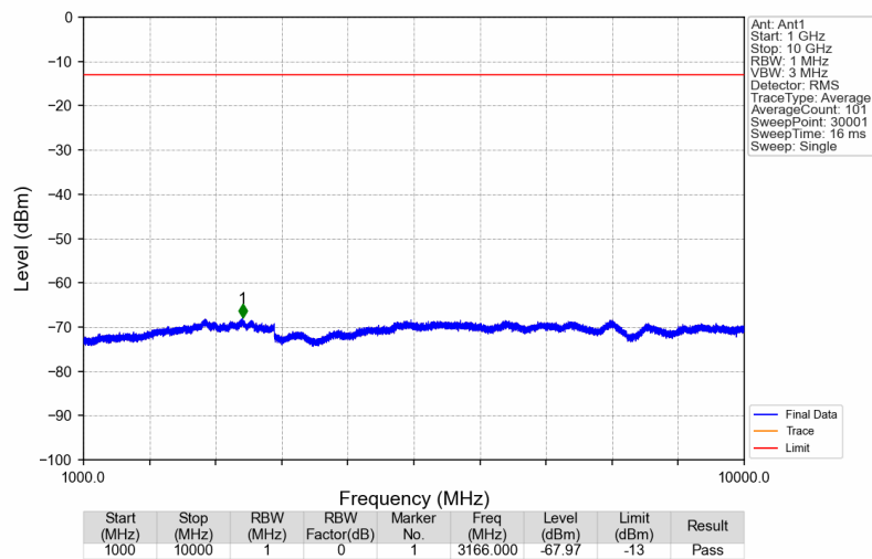
Band13_748.5MHz_AWGN_SISO_Ant1_NTNV
