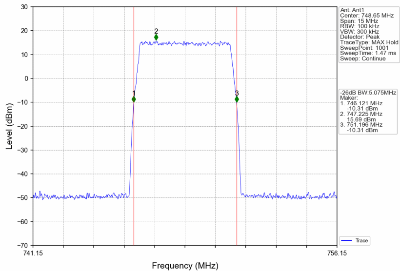
Band13_748.65MHz_AWGN_SISO_Ant1_NTNV_AGC
