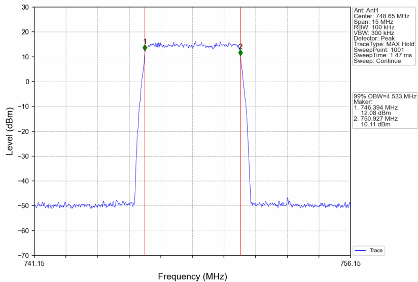
Band13_748.65MHz_AWGN_SISO_Ant1_NTNV_AGC
