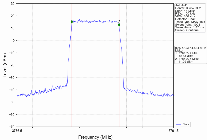
3780MHz-3980MHz_3784MHz_AWGN_SISO_Ant1_NTNV_AGC
