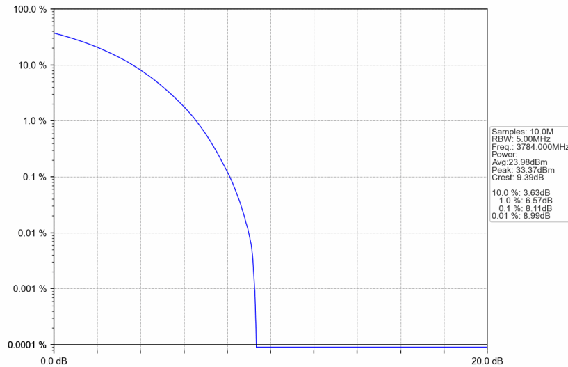
3780MHz-3980MHz_3784MHz_AWGN_SISO_Ant1_NTNV_AGC+3
