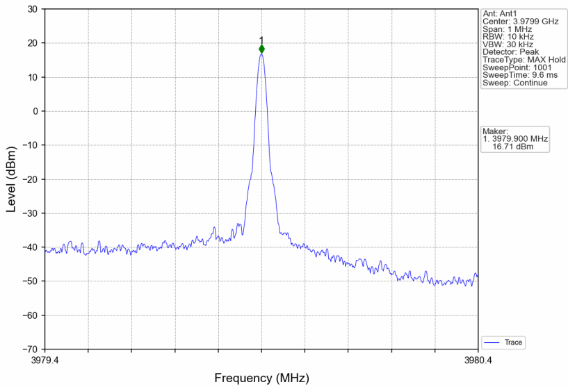
3780MHz-3980MHz_3979.9MHz_CW_SISO_Ant1_NTNV
