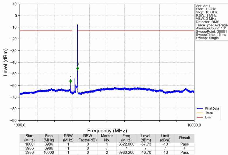
3780MHz-3980MHz_3977.5MHz_AWGN_SISO_Ant1_NTNV
