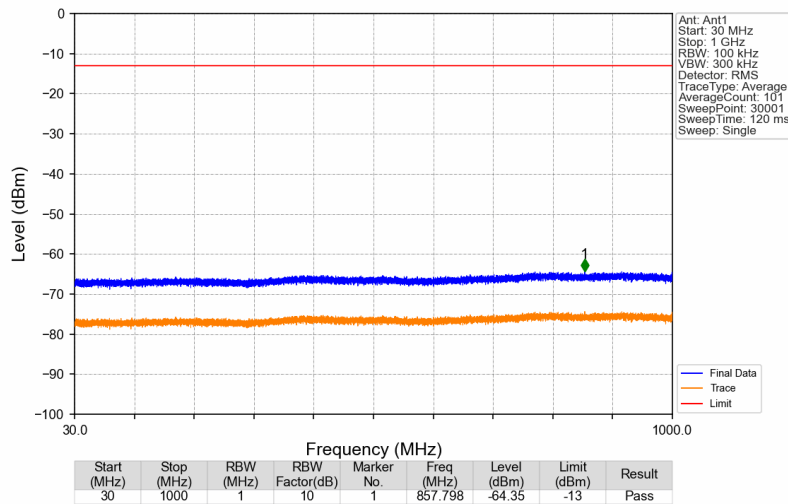
3780MHz-3980MHz_3977.5MHz_AWGN_SISO_Ant1_NTNV
