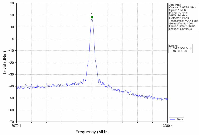
3780MHz-3980MHz_3979.9MHz_CW_SISO_Ant1_NTNV
