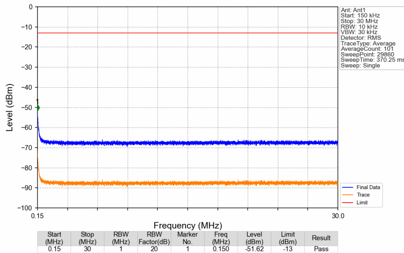
3780MHz-3980MHz_3977.5MHz_AWGN_SISO_Ant1_NTNV
