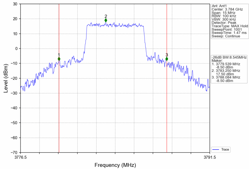
3780MHz-3980MHz_3784MHz_AWGN_SISO_Ant1_NTNV_AGC+3
