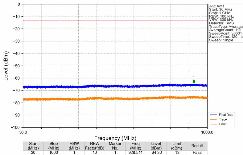
3780MHz-3980MHz_3782.5MHz_AWGN_SISO_Ant1_NTNV
