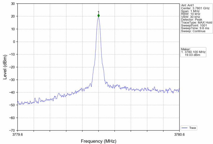
3780MHz-3980MHz_3780.1MHz_CW_SISO_Ant1_NTNV
