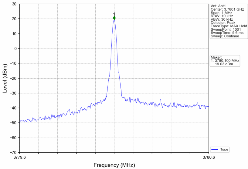
3780MHz-3980MHz_3780.1MHz_CW_SISO_Ant1_NTNV
