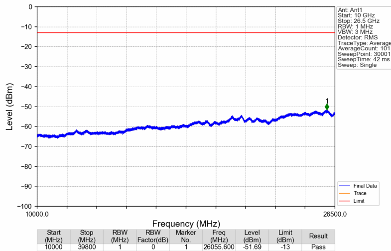
3780MHz-3980MHz_3977.5MHz_AWGN_SISO_Ant1_NTNV
