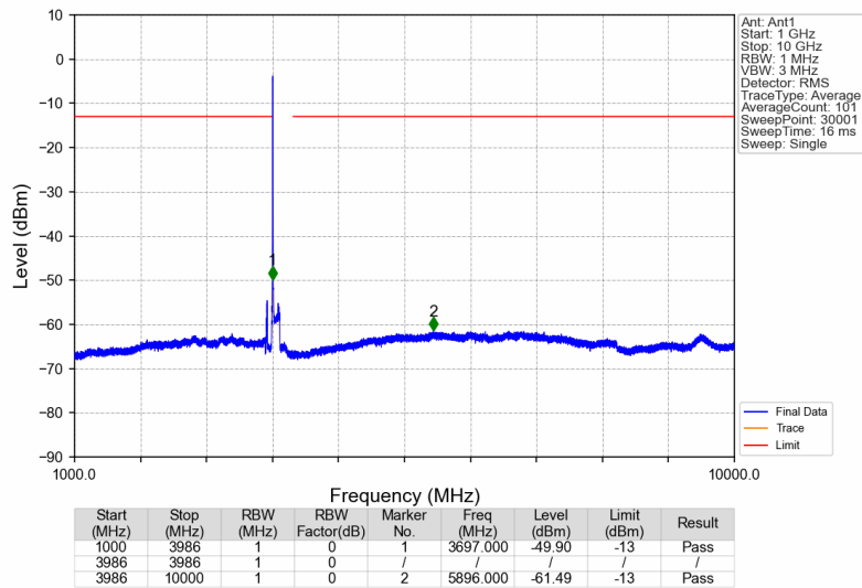
3700MHz-3900MHz_3702.5MHz_AWGN_SISO_Ant1_NTNV
