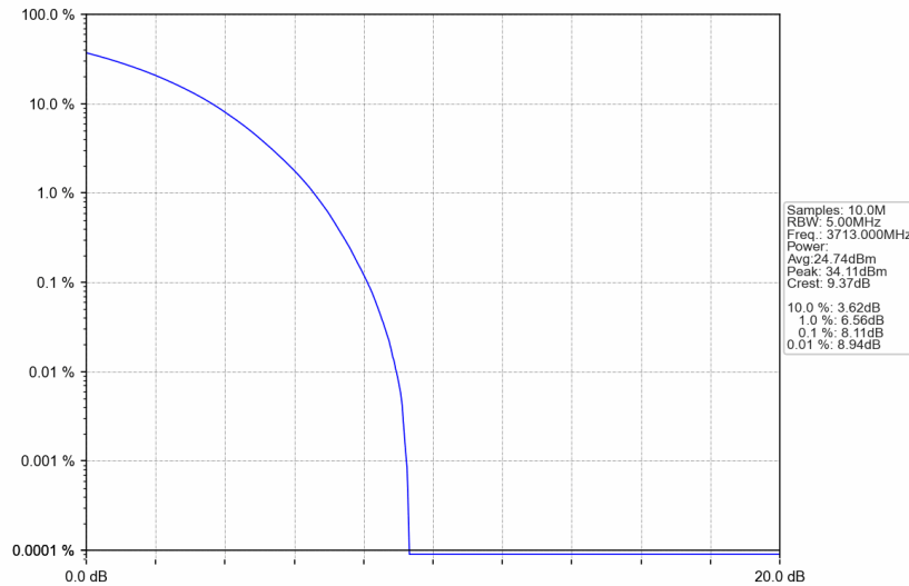
3700MHz-3900MHz_3713MHz_AWGN_SISO_Ant1_NTNV_AGC+3
