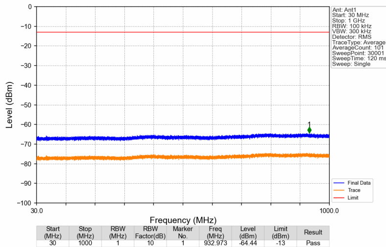
3700MHz-3900MHz_3702.5MHz_AWGN_SISO_Ant1_NTNV
