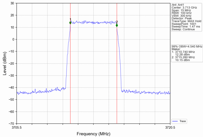
3700MHz-3900MHz_3713MHz_AWGN_SISO_Ant1_NTNV_AGC
