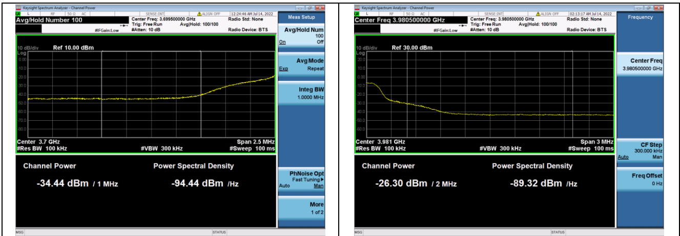
5G NR Band n77 _ SCS 30K Intra-band Continuous CA, Nominal Bandwidth: 10M+10M _ Low channel+ High channel
