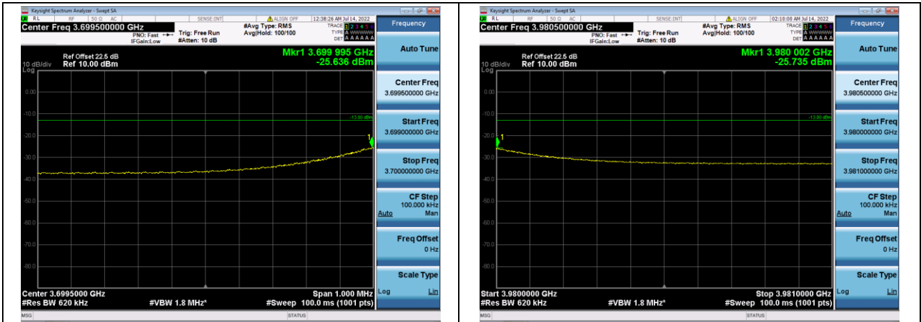
5G NR Band n77 _ SCS 30K, Nominal Bandwidth: 80M _ Low channel+ High channel
