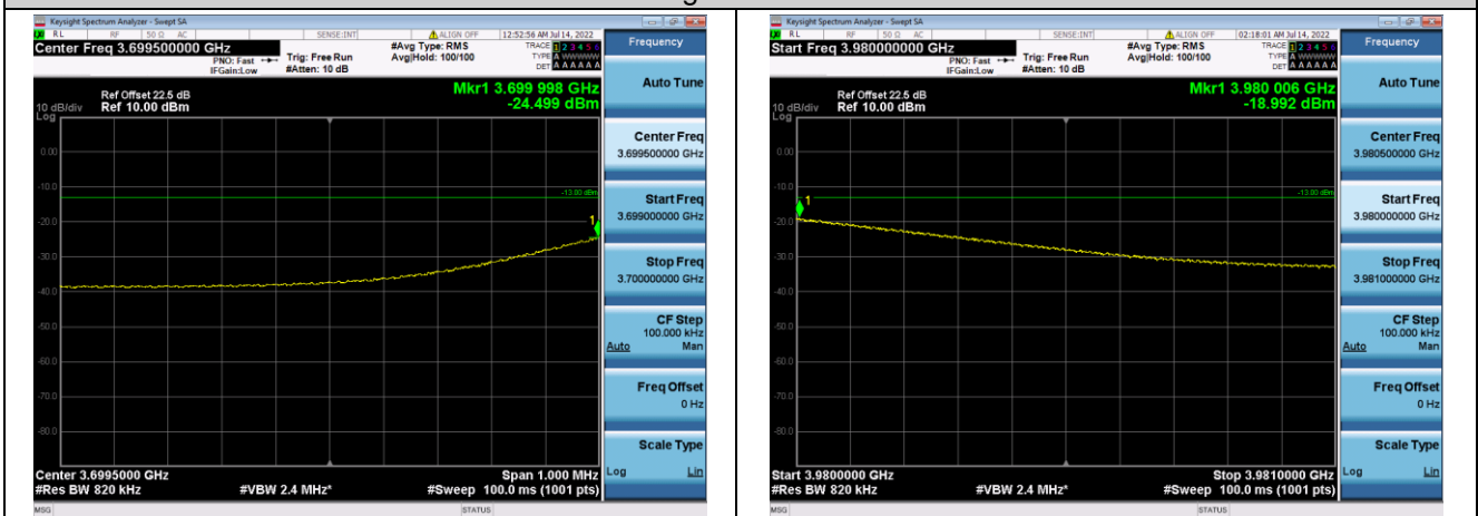
5G NR Band n77 _ SCS 30K Intra-band Continuous CA, Nominal Bandwidth: 60M+60M+60M _ Low channel+ High channel
