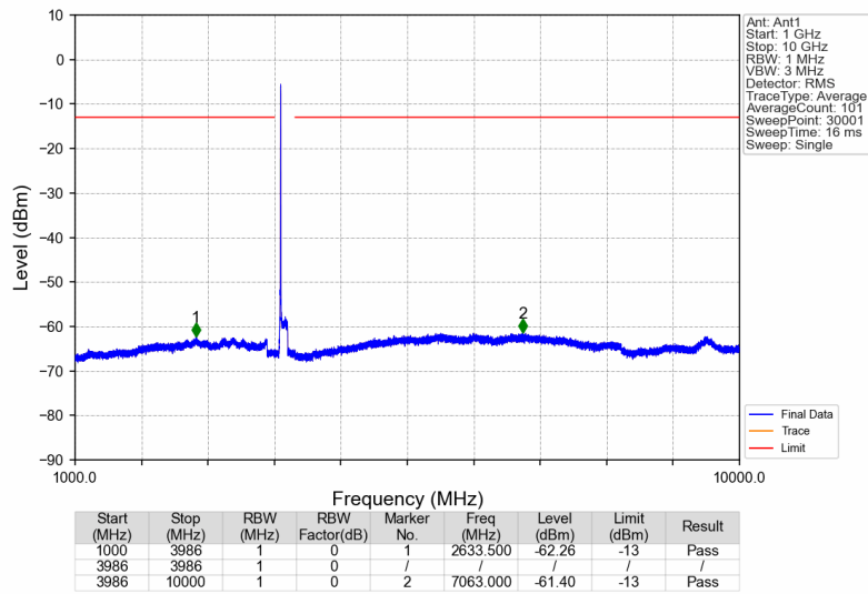
3780MHz-3980MHz_3782.5MHz_AWGN_SISO_Ant1_NTNV
