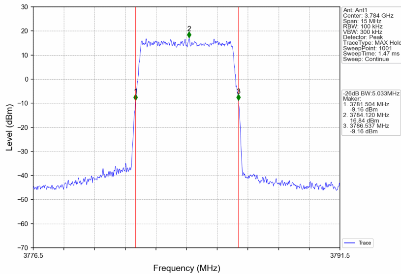
3780MHz-3980MHz_3784MHz_AWGN_SISO_Ant1_NTNV_AGC+3
