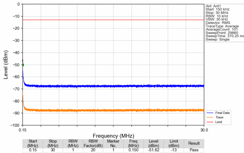
3780MHz-3980MHz_3977.5MHz_AWGN_SISO_Ant1_NTNV
