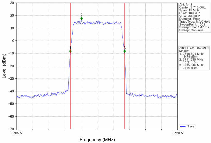
3700MHz-3900MHz_3713MHz_AWGN_SISO_Ant1_NTNV_AGC
