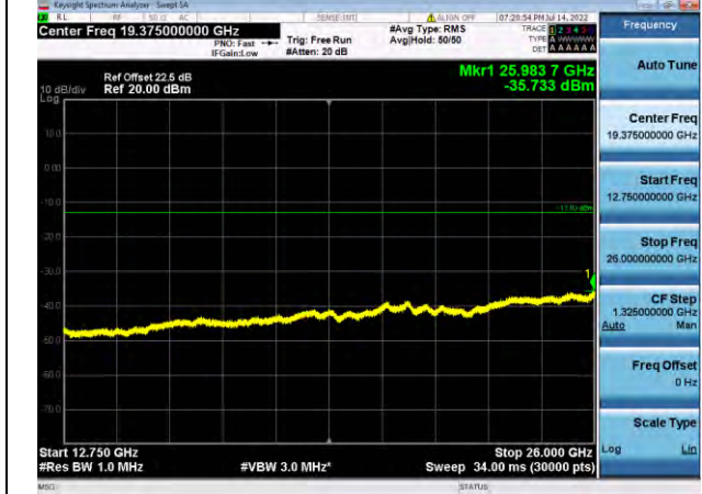
QPSK Low channel - 12.75GHz~26GHz
