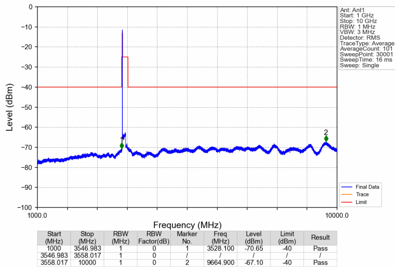
3550MHz-3700MHz_3552.5MHz_AWGN_SISO_Ant1_NTNV
