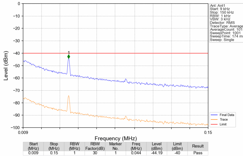
3550MHz-3700MHz_3625MHz_AWGN_SISO_Ant1_NTNV
