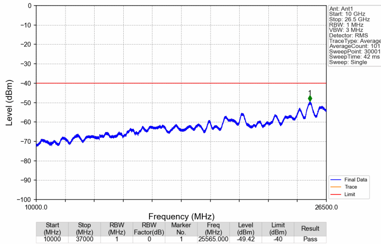
3550MHz-3700MHz_3697.5MHz_AWGN_SISO_Ant1_NTNV
