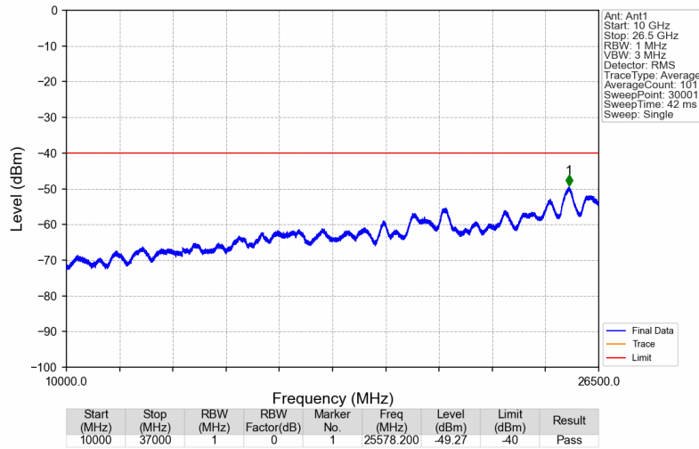
3550MHz-3700MHz_3552.5MHz_AWGN_SISO_Ant1_NTNV
