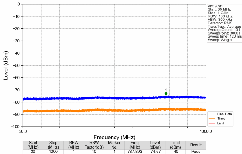
3550MHz-3700MHz_3697.5MHz_AWGN_SISO_Ant1_NTNV
