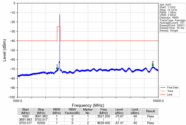
3550MHz-3700MHz_3697.5MHz_AWGN_SISO_Ant1_NTNV
