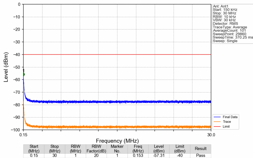
3550MHz-3700MHz_3697.5MHz_AWGN_SISO_Ant1_NTNV
