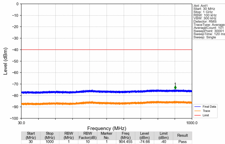
3550MHz-3700MHz_3552.5MHz_AWGN_SISO_Ant1_NTNV
