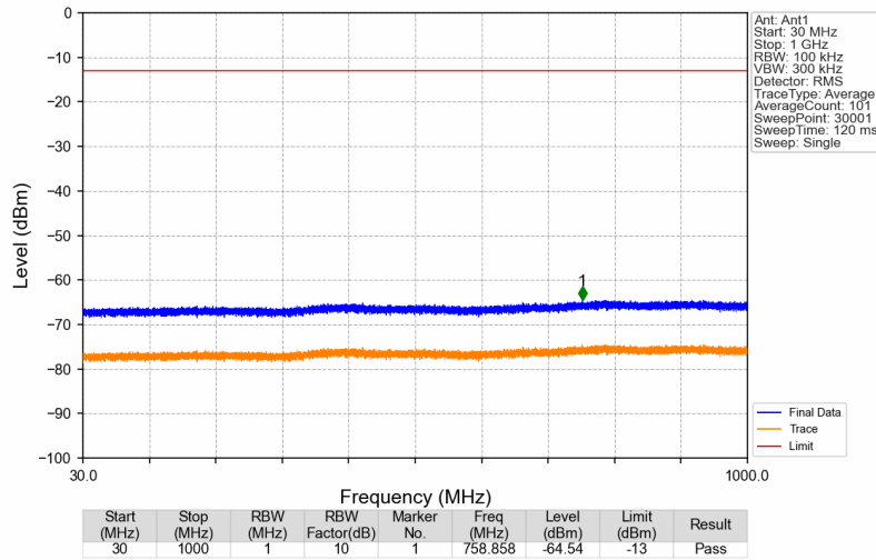
3700MHz-3800MHz_3797.5MHz_AWGN_SISO_Ant1_NTNV
