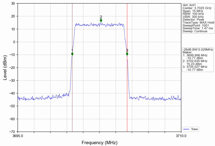
3700MHz-3800MHz_3702.5MHz_AWGN_SISO_Ant1_NTNV_AGC
