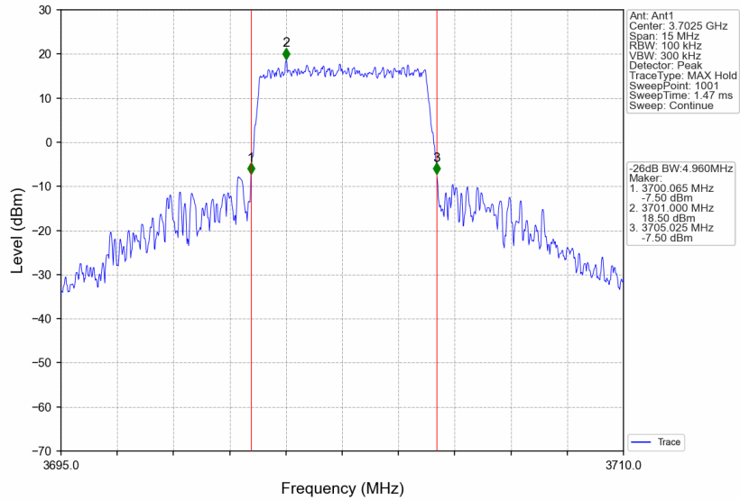
3700MHz-3800MHz_3702.5MHz_AWGN_SISO_Ant1_NTNV_AGC+3
