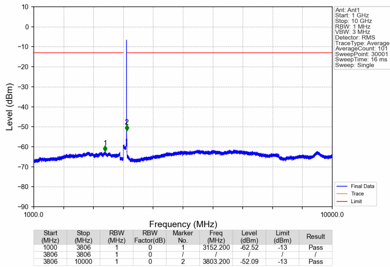
3700MHz-3800MHz_3797.5MHz_AWGN_SISO_Ant1_NTNV
