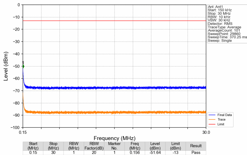
3700MHz-3800MHz_3797.5MHz_AWGN_SISO_Ant1_NTNV
