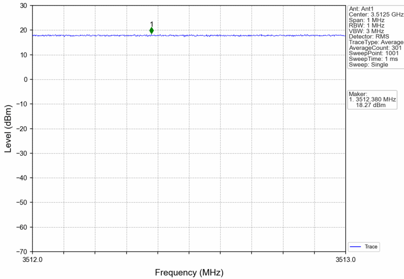
3450MHz-3550MHz_3512.5MHz_GMSK_SISO_Ant1_NTNV_AGC+3
