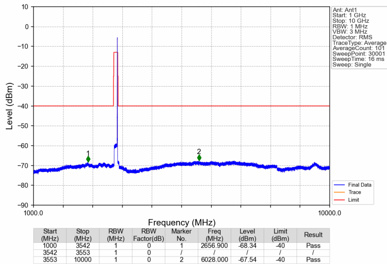
3450MHz-3550MHz_3547.5MHz_AWGN_SISO_Ant1_NTNV
