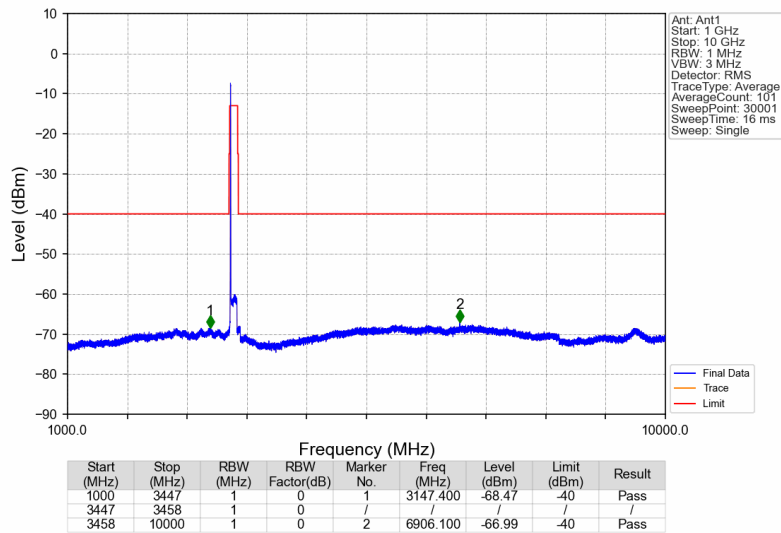
3450MHz-3550MHz_3452.5MHz_AWGN_SISO_Ant1_NTNV
