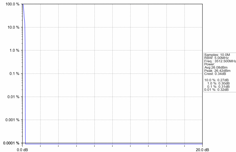
3450MHz-3550MHz_3512.5MHz_GMSK_SISO_Ant1_NTNV_AGC+3
