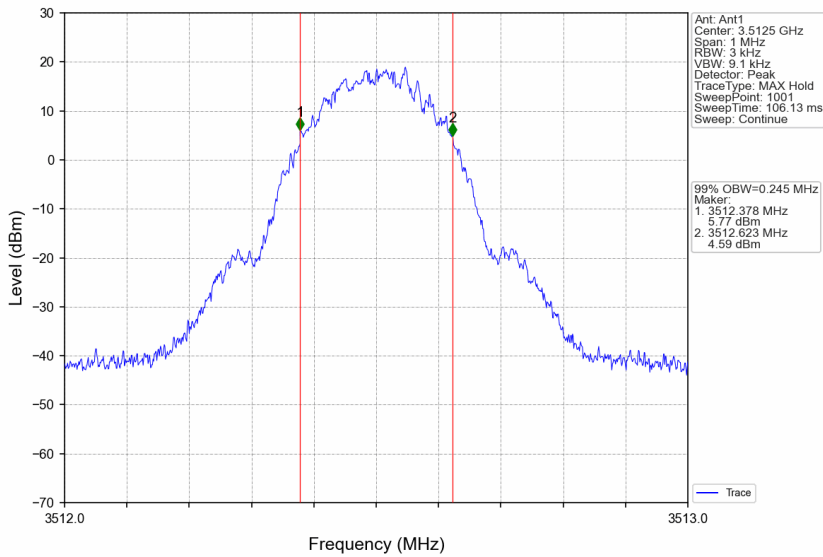
3450MHz-3550MHz_3512.5MHz_GMSK_SISO_Ant1_NTNV_AGC+3
