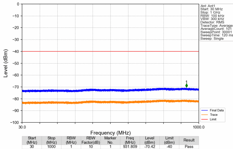
3450MHz-3550MHz_3500MHz_AWGN_SISO_Ant1_NTNV
