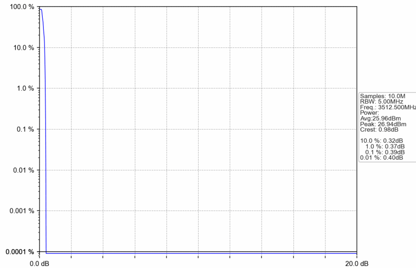
3450MHz-3550MHz_3512.5MHz_GMSK_SISO_Ant1_NTNV_AGC
