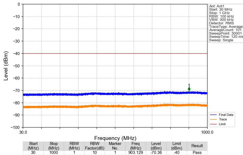
3450MHz-3550MHz_3452.5MHz_AWGN_SISO_Ant1_NTNV
