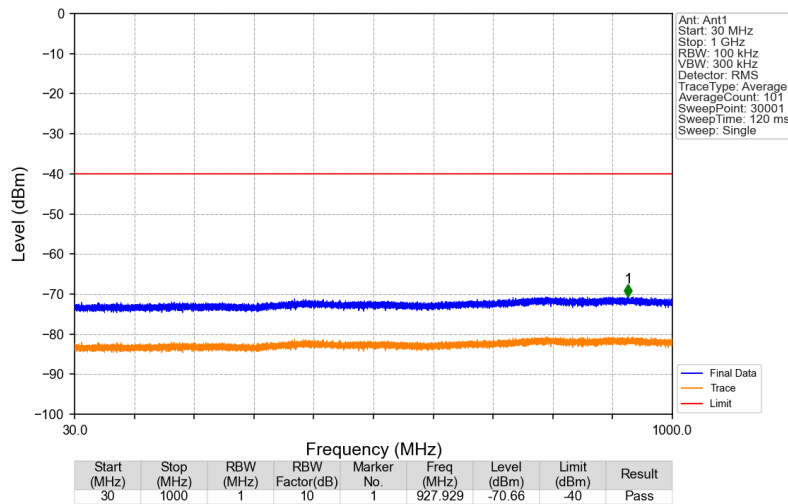
3450MHz-3550MHz_3547.5MHz_AWGN_SISO_Ant1_NTNV
