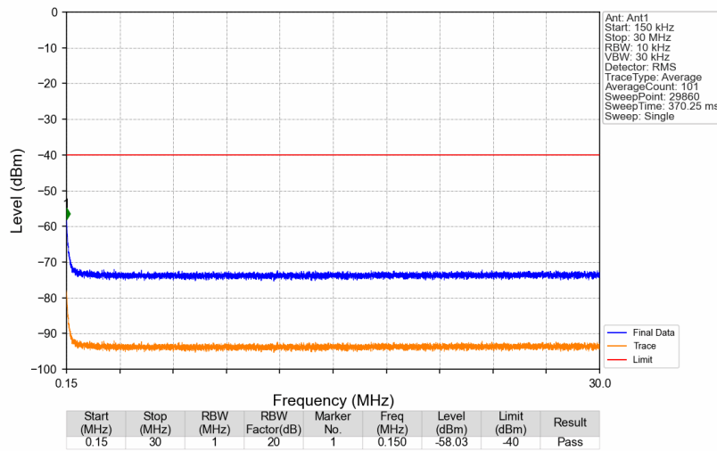
3450MHz-3550MHz_3547.5MHz_AWGN_SISO_Ant1_NTNV
