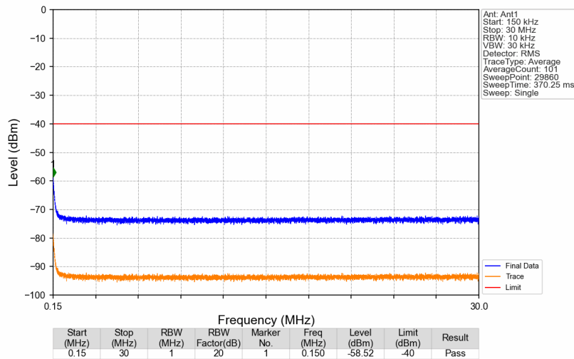
3450MHz-3550MHz_3500MHz_AWGN_SISO_Ant1_NTNV
