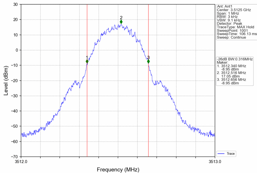
3450MHz-3550MHz_3512.5MHz_GMSK_SISO_Ant1_NTNV_AGC
