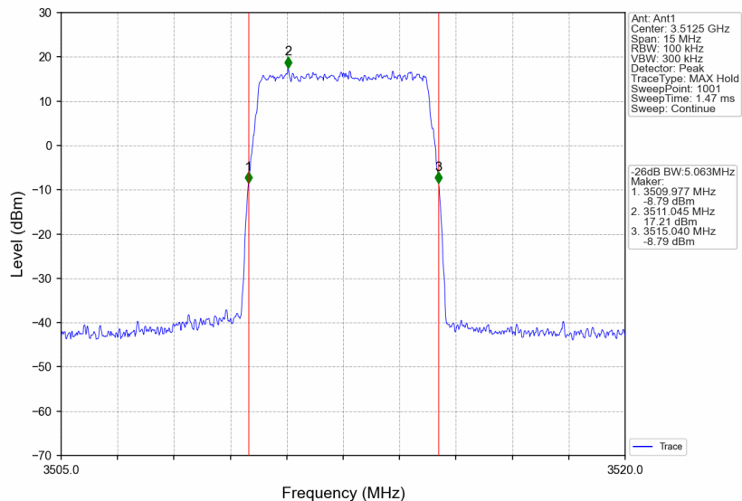
3450MHz-3550MHz_3512.5MHz_AWGN_SISO_Ant1_NTNV_AGC
