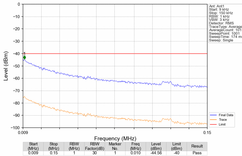
3450MHz-3550MHz_3500MHz_AWGN_SISO_Ant1_NTNV
