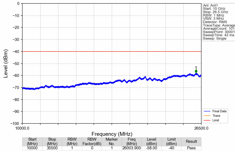
3450MHz-3550MHz_3547.5MHz_AWGN_SISO_Ant1_NTNV
