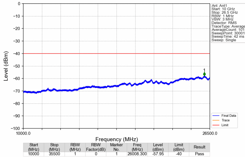
3450MHz-3550MHz_3452.5MHz_AWGN_SISO_Ant1_NTNV
