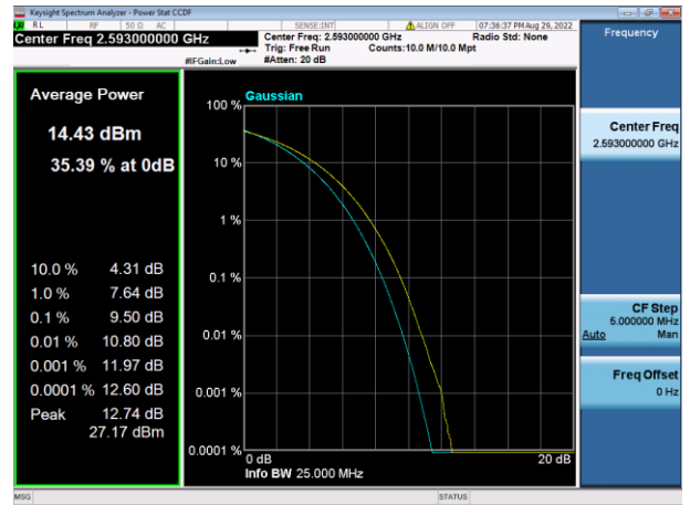
QPSK Middle channel
