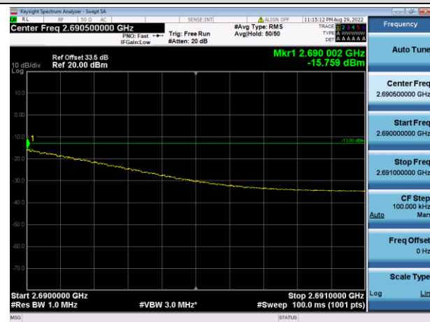
5G NR Band n41 Carrier 1CC, SCS 30K, Contiguous CA, Bandwidth:100M Channel 2640MHz
