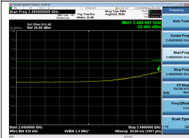
5G NR Band n41 Carrier 3CC, SCS 30K, Contiguous CA, Bandwidth:60+60+60M Channel 2526+2586+2646MHz
