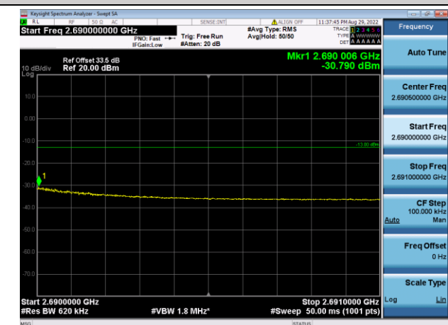
5G NR Band n41 Carrier 3CC, SCS 30K, Contiguous CA, Bandwidth:60+60+60M Channel 2540+2600+2660MHz
