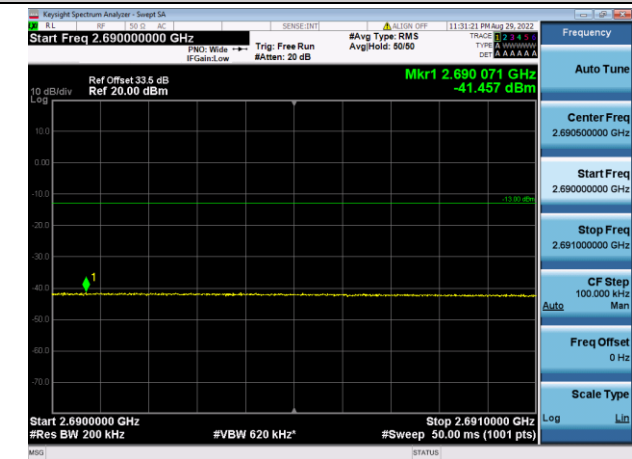
5G NR Band n41 Carrier 2CC, SCS 30K, Contiguous CA, Bandwidth:80+80M Channel 2570+2650MHz
