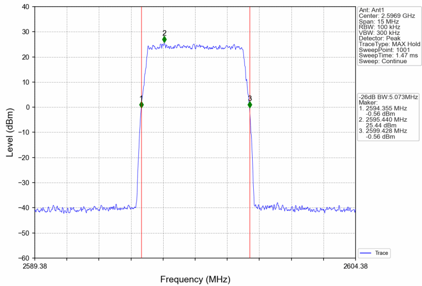
Band41_2596.88MHz_AWGN_SISO_Ant1_NTNV_AGC
