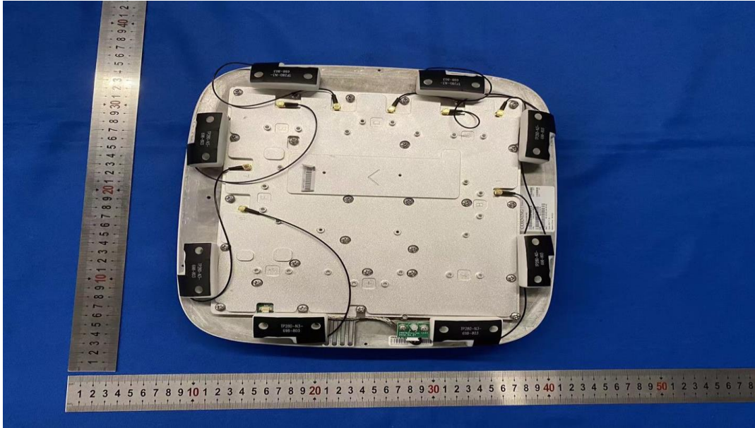
Internal Antenna
