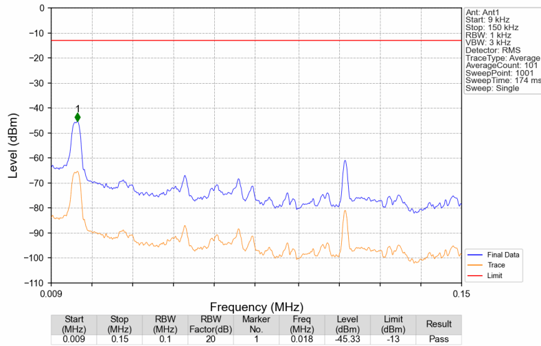
Band71_634.5MHz_AWGN_SISO_Ant1_NTNV
