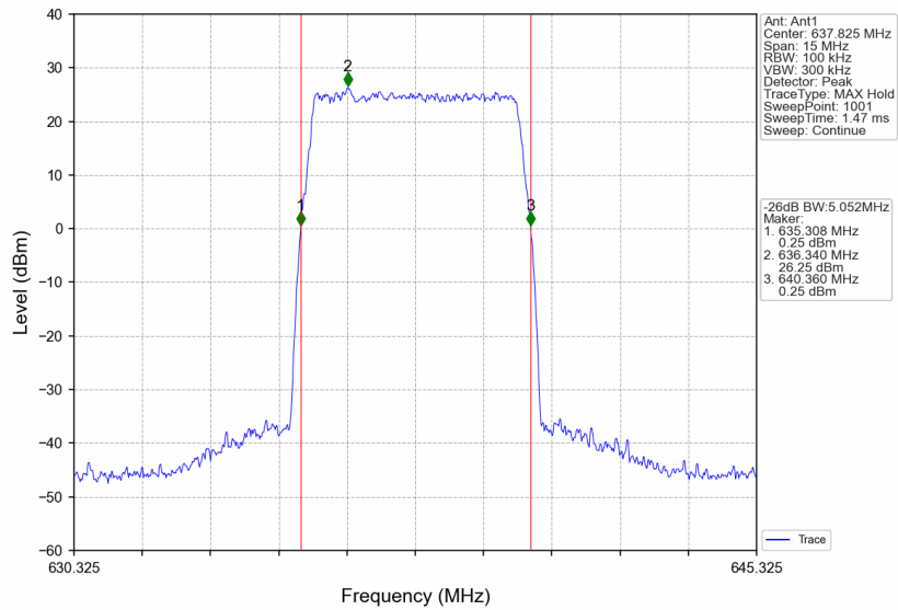
Band71_637.825MHz_AWGN_SISO_Ant1_NTNV_AGC
