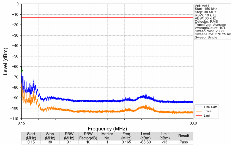
Band71_634.5MHz_AWGN_SISO_Ant1_NTNV
