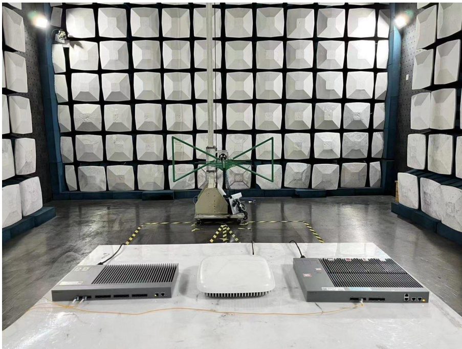
Radiated Spurious Emissions (30MHz-1GHz)
